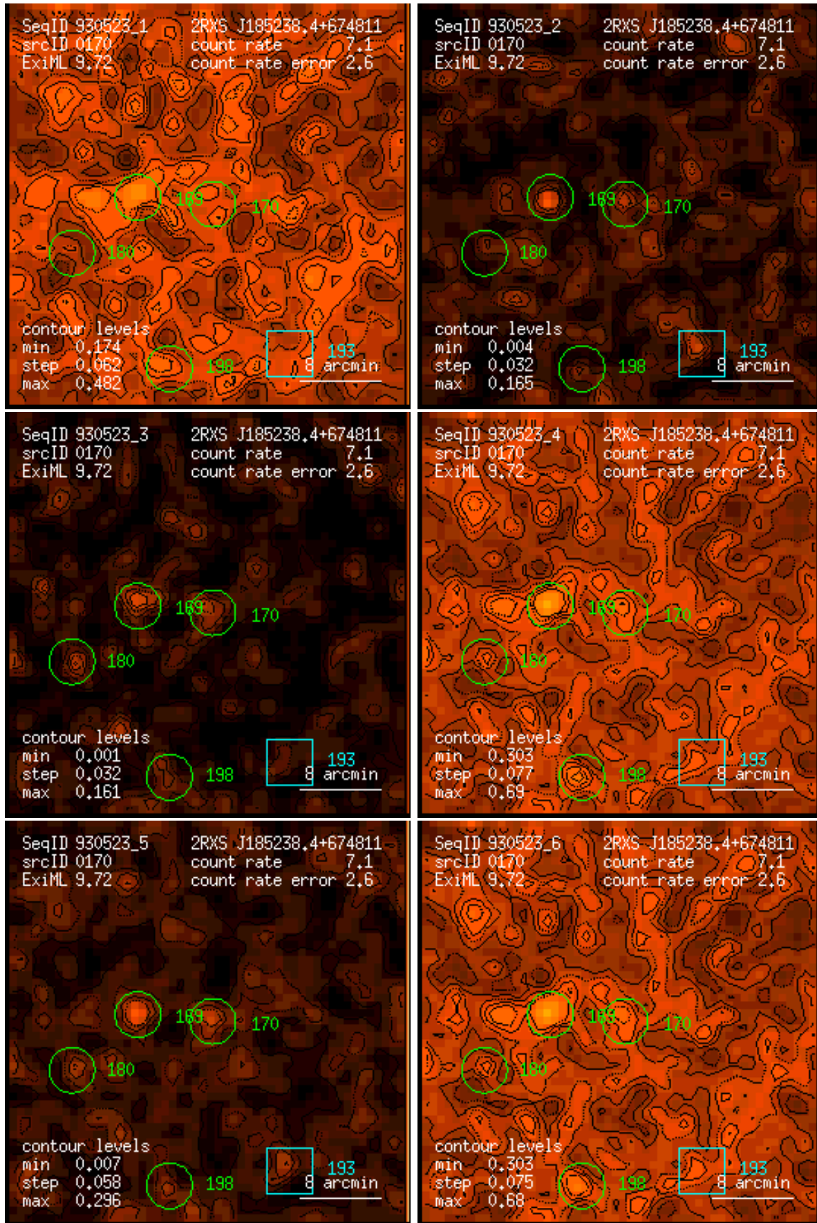
Figure 170: RASS 930523: detection 0170: band rate images, Gaussian filter: (1) PSPC channels 11 – 41, (2) 52 – 90, (3) 91 – 201, (4) 11 – 235, (5) 52 – 201, (6) 11 – 201. Broad band rates in counts/ks. Band rate contour levels in counts/ks/arcmin 2 .
