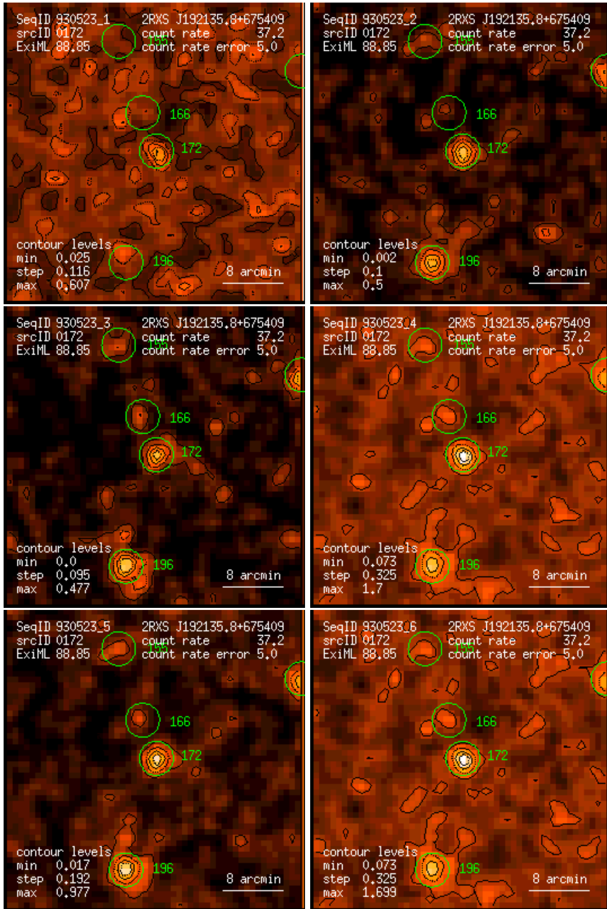
Figure 172: RASS 930523: detection 0172: band rate images, Gaussian filter: (1) PSPC channels 11 – 41, (2) 52 – 90, (3) 91 – 201, (4) 11 – 235, (5) 52 – 201, (6) 11 – 201. Broad band rates in counts/ks. Band rate contour levels in counts/ks/arcmin 2 .
