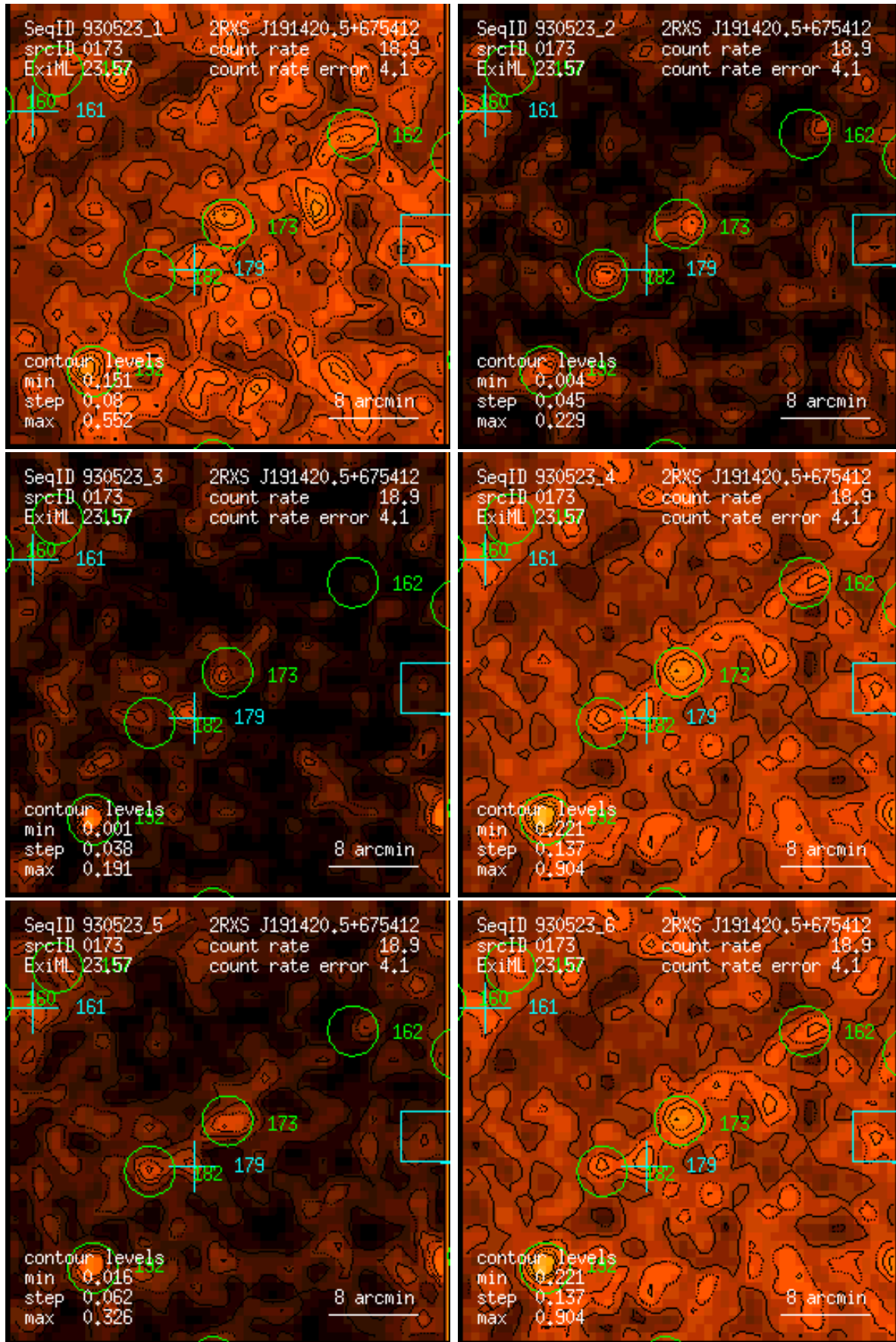
Figure 173: RASS 930523: detection 0173: band rate images, Gaussian filter: (1) PSPC channels 11 – 41, (2) 52 – 90, (3) 91 – 201, (4) 11 – 235, (5) 52 – 201, (6) 11 – 201. Broad band rates in counts/ks. Band rate contour levels in counts/ks/arcmin 2 .
