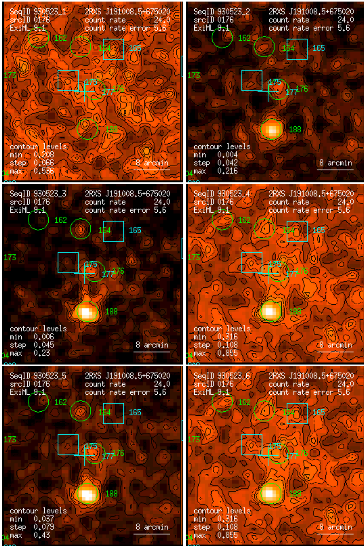
Figure 176: RASS 930523: detection 0176: band rate images, Gaussian filter: (1) PSPC channels 11 – 41, (2) 52 – 90, (3) 91 – 201, (4) 11 – 235, (5) 52 – 201, (6) 11 – 201. Broad band rates in counts/ks. Band rate contour levels in counts/ks/arcmin 2 .
