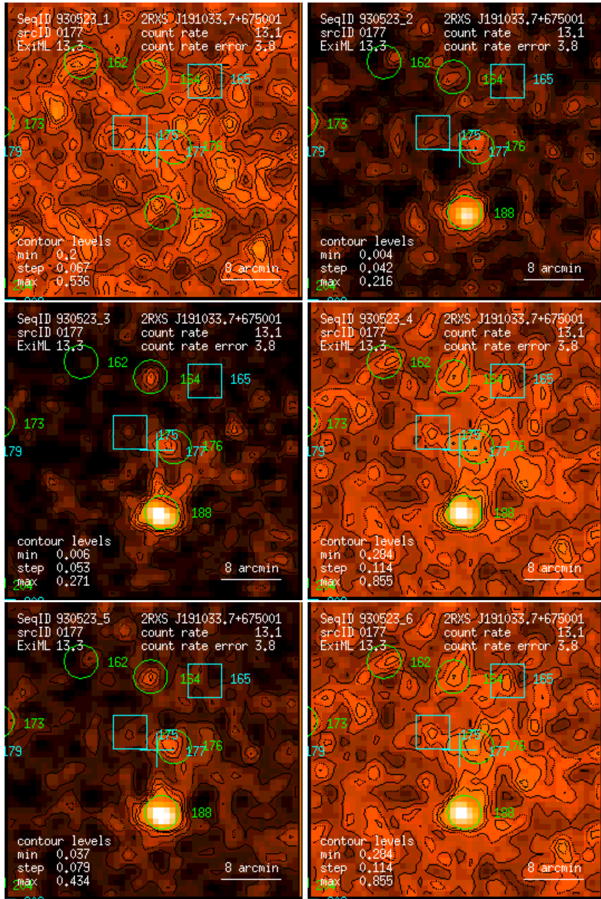
Figure 177: RASS 930523: detection 0177: band rate images, Gaussian filter: (1) PSPC channels 11 – 41, (2) 52 – 90, (3) 91 – 201, (4) 11 – 235, (5) 52 – 201, (6) 11 – 201. Broad band rates in counts/ks. Band rate contour levels in counts/ks/arcmin 2 .
