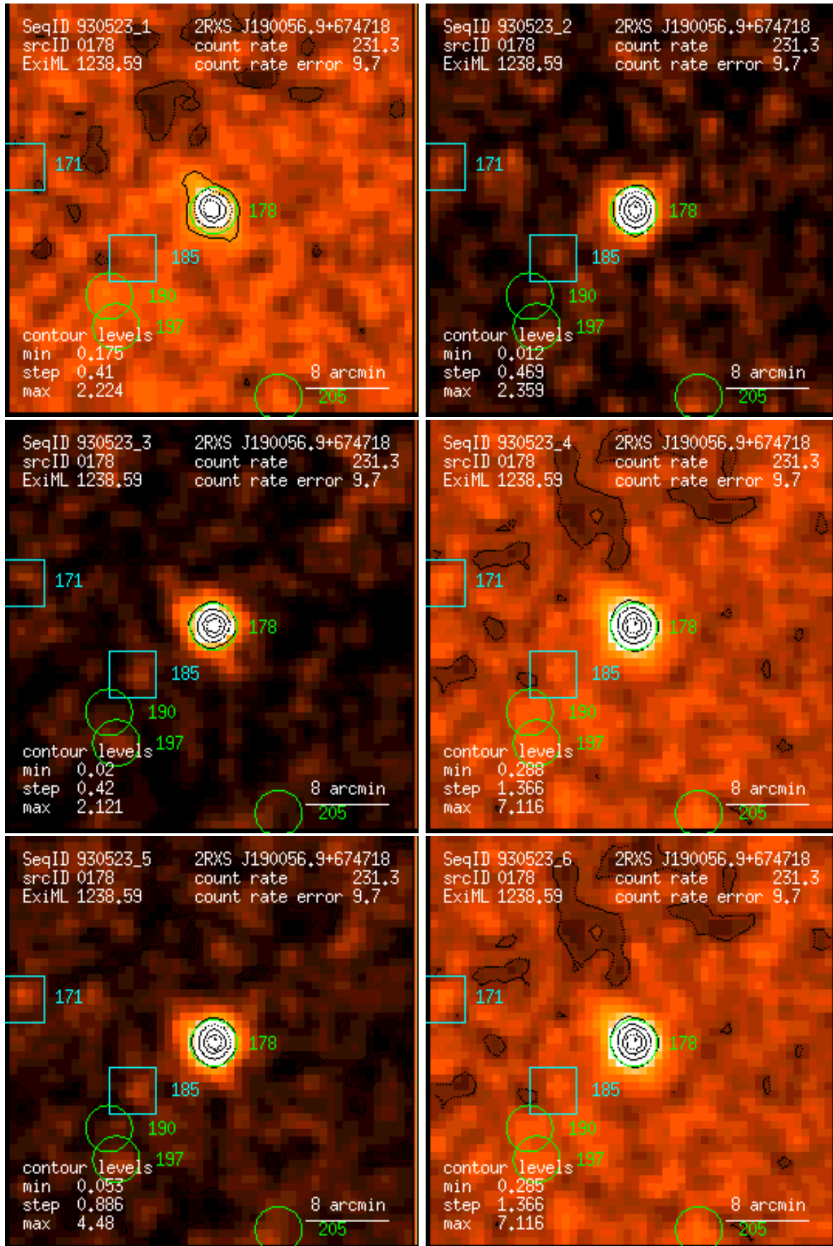
Figure 178: RASS 930523: detection 0178: band rate images, Gaussian filter: (1) PSPC channels 11 – 41, (2) 52 – 90, (3) 91 – 201, (4) 11 – 235, (5) 52 – 201, (6) 11 – 201. Broad band rates in counts/ks. Band rate contour levels in counts/ks/arcmin 2 .
