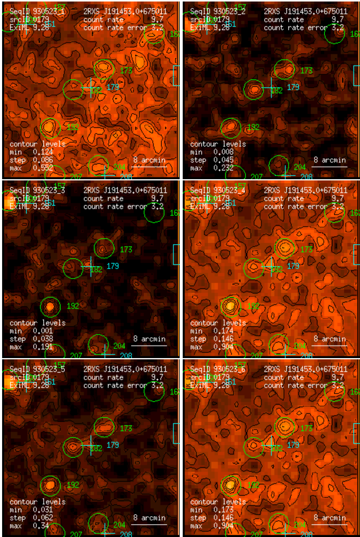
Figure 179: RASS 930523: detection 0179: band rate images, Gaussian filter: (1) PSPC channels 11 – 41, (2) 52 – 90, (3) 91 – 201, (4) 11 – 235, (5) 52 – 201, (6) 11 – 201. Broad band rates in counts/ks. Band rate contour levels in counts/ks/arcmin 2 .
