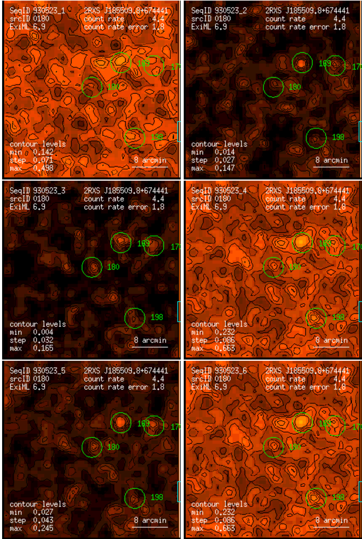
Figure 180: RASS 930523: detection 0180: band rate images, Gaussian filter: (1) PSPC channels 11 – 41, (2) 52 – 90, (3) 91 – 201, (4) 11 – 235, (5) 52 – 201, (6) 11 – 201. Broad band rates in counts/ks. Band rate contour levels in counts/ks/arcmin 2 .
