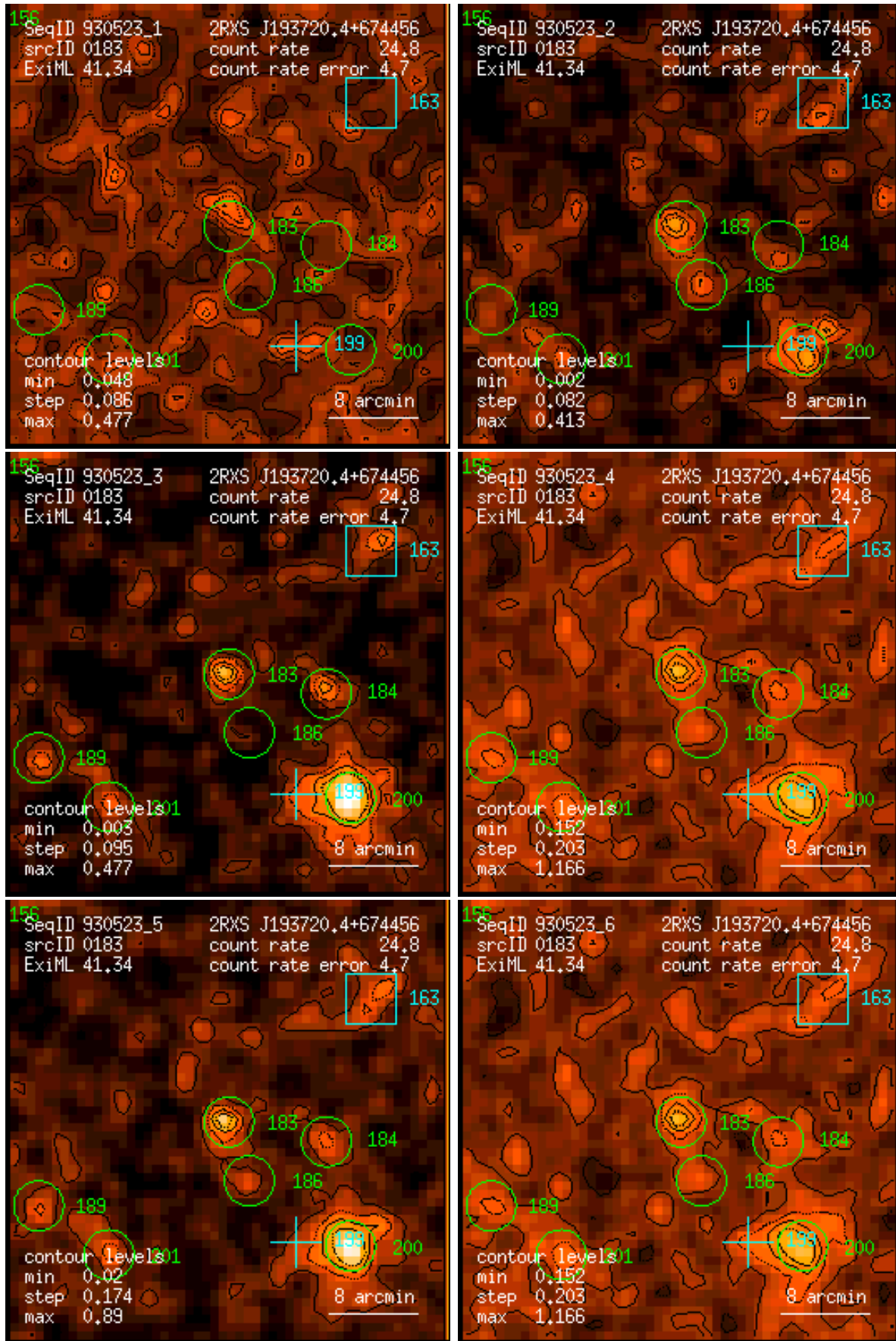
Figure 183: RASS 930523: detection 0183: band rate images, Gaussian filter: (1) PSPC channels 11 – 41, (2) 52 – 90, (3) 91 – 201, (4) 11 – 235, (5) 52 – 201, (6) 11 – 201. Broad band rates in counts/ks. Band rate contour levels in counts/ks/arcmin 2 .
