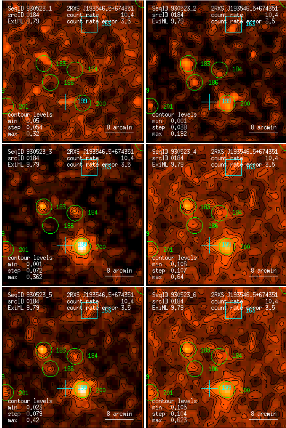
Figure 184: RASS 930523: detection 0184: band rate images, Gaussian filter: (1) PSPC channels 11 – 41, (2) 52 – 90, (3) 91 – 201, (4) 11 – 235, (5) 52 – 201, (6) 11 – 201. Broad band rates in counts/ks. Band rate contour levels in counts/ks/arcmin 2 .
