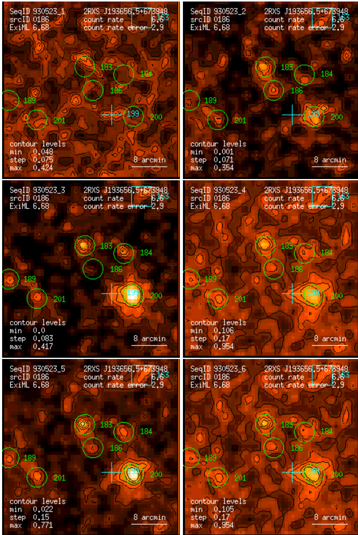
Figure 186: RASS 930523: detection 0186: band rate images, Gaussian filter: (1) PSPC channels 11 – 41, (2) 52 – 90, (3) 91 – 201, (4) 11 – 235, (5) 52 – 201, (6) 11 – 201. Broad band rates in counts/ks. Band rate contour levels in counts/ks/arcmin 2 .
