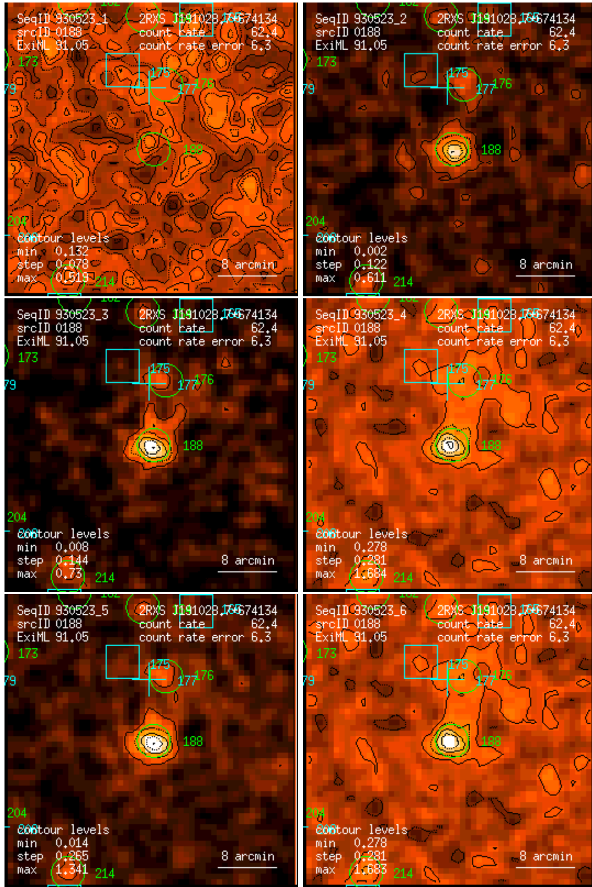
Figure 188: RASS 930523: detection 0188: band rate images, Gaussian filter: (1) PSPC channels 11 – 41, (2) 52 – 90, (3) 91 – 201, (4) 11 – 235, (5) 52 – 201, (6) 11 – 201. Broad band rates in counts/ks. Band rate contour levels in counts/ks/arcmin 2 .
