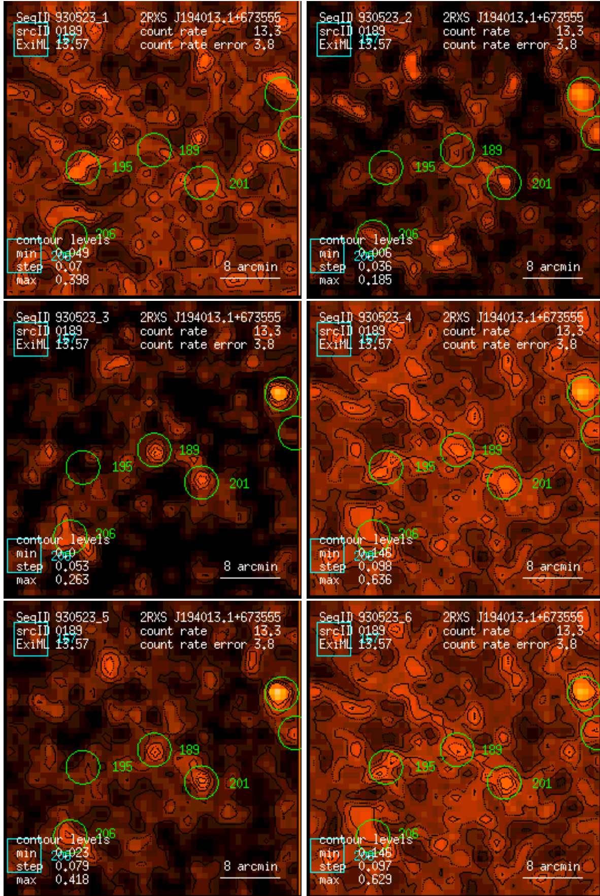
Figure 189: RASS 930523: detection 0189: band rate images, Gaussian filter: (1) PSPC channels 11 – 41, (2) 52 – 90, (3) 91 – 201, (4) 11 – 235, (5) 52 – 201, (6) 11 – 201. Broad band rates in counts/ks. Band rate contour levels in counts/ks/arcmin 2 .
