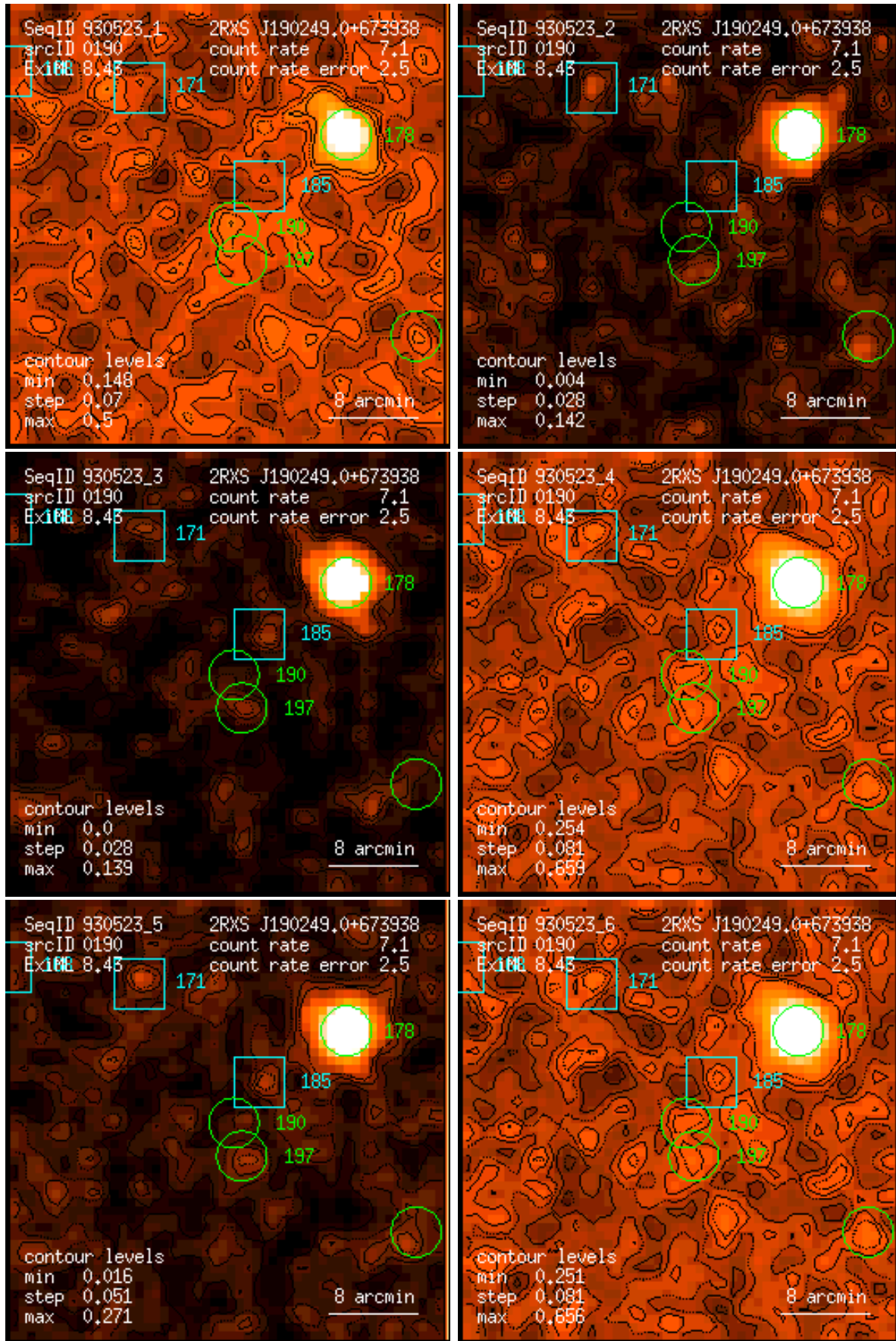
Figure 190: RASS 930523: detection 0190: band rate images, Gaussian filter: (1) PSPC channels 11 – 41, (2) 52 – 90, (3) 91 – 201, (4) 11 – 235, (5) 52 – 201, (6) 11 – 201. Broad band rates in counts/ks. Band rate contour levels in counts/ks/arcmin 2 .
