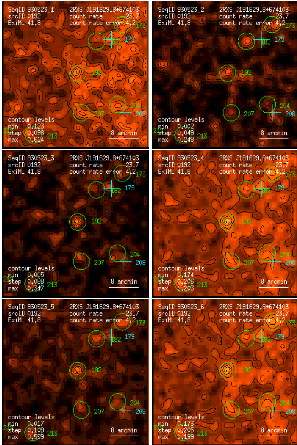
Figure 192: RASS 930523: detection 0192: band rate images, Gaussian filter: (1) PSPC channels 11 – 41, (2) 52 – 90, (3) 91 – 201, (4) 11 – 235, (5) 52 – 201, (6) 11 – 201. Broad band rates in counts/ks. Band rate contour levels in counts/ks/arcmin 2 .
