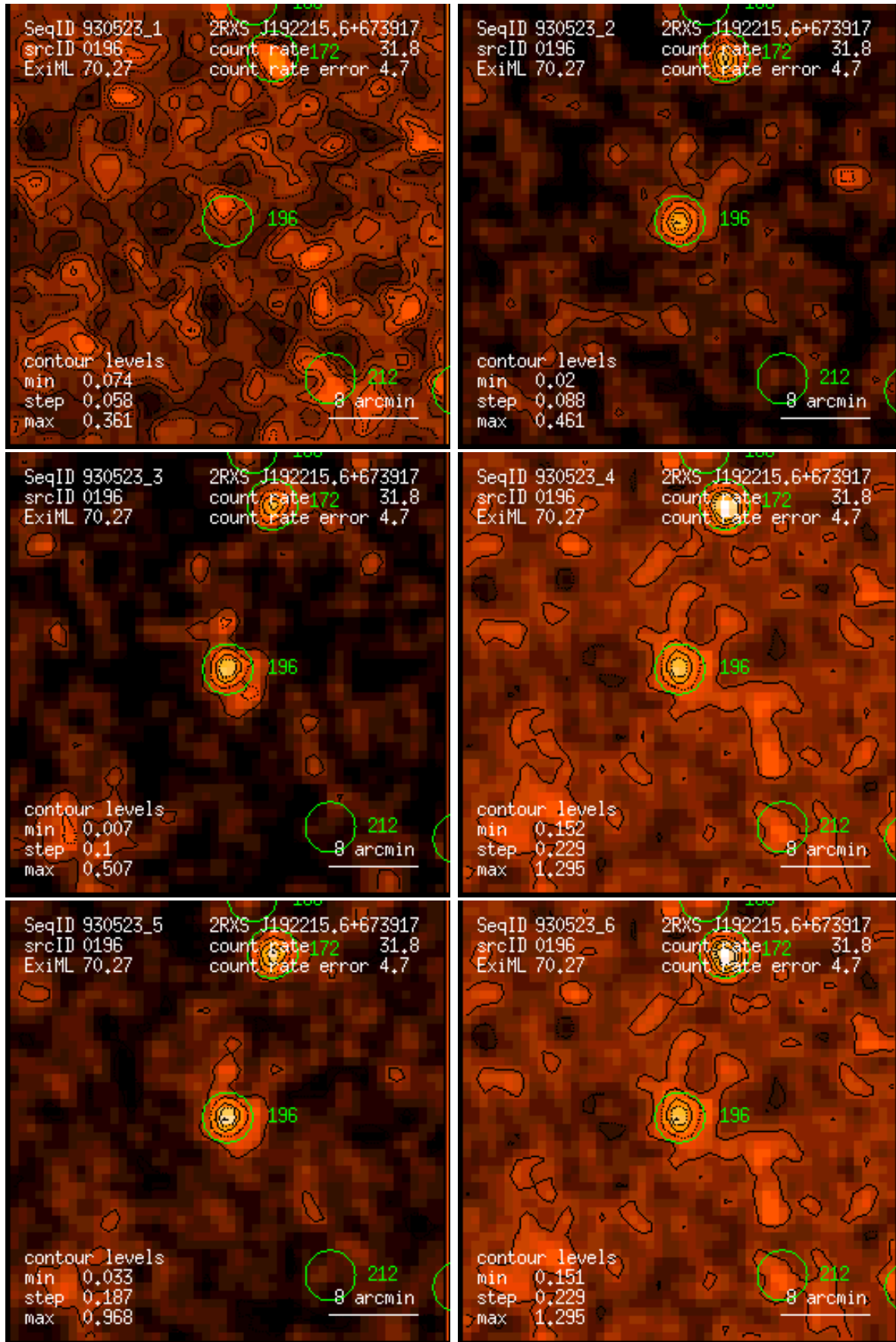
Figure 196: RASS 930523: detection 0196: band rate images, Gaussian filter: (1) PSPC channels 11 – 41, (2) 52 – 90, (3) 91 – 201, (4) 11 – 235, (5) 52 – 201, (6) 11 – 201. Broad band rates in counts/ks. Band rate contour levels in counts/ks/arcmin 2 .
