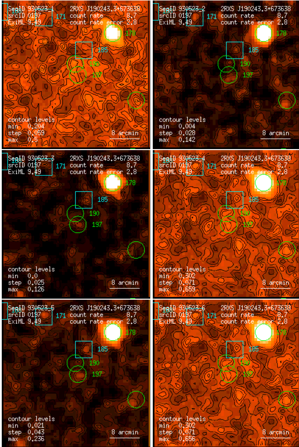
Figure 197: RASS 930523: detection 0197: band rate images, Gaussian filter: (1) PSPC channels 11 – 41, (2) 52 – 90, (3) 91 – 201, (4) 11 – 235, (5) 52 – 201, (6) 11 – 201. Broad band rates in counts/ks. Band rate contour levels in counts/ks/arcmin 2 .
