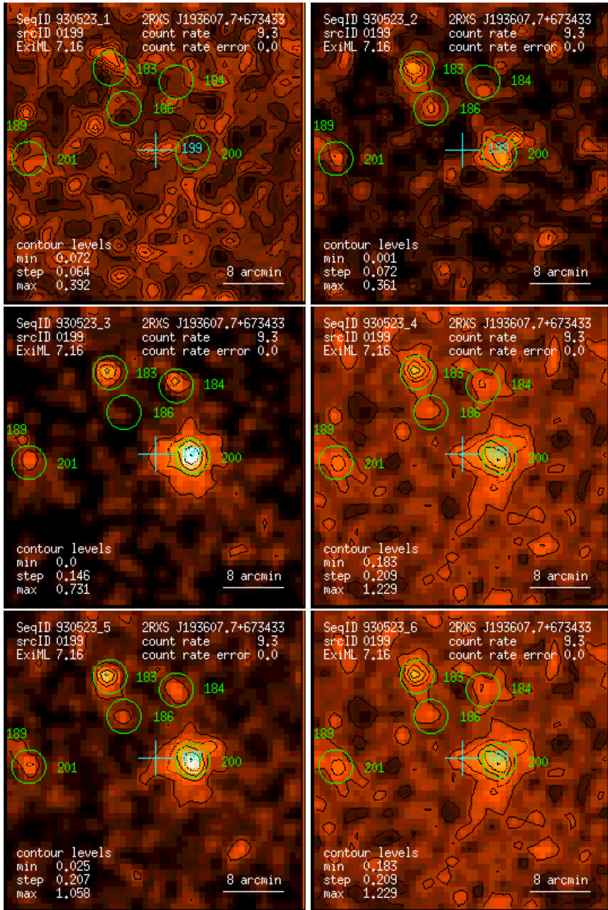
Figure 199: RASS 930523: detection 0199: band rate images, Gaussian filter: (1) PSPC channels 11 – 41, (2) 52 – 90, (3) 91 – 201, (4) 11 – 235, (5) 52 – 201, (6) 11 – 201. Broad band rates in counts/ks. Band rate contour levels in counts/ks/arcmin 2 .
