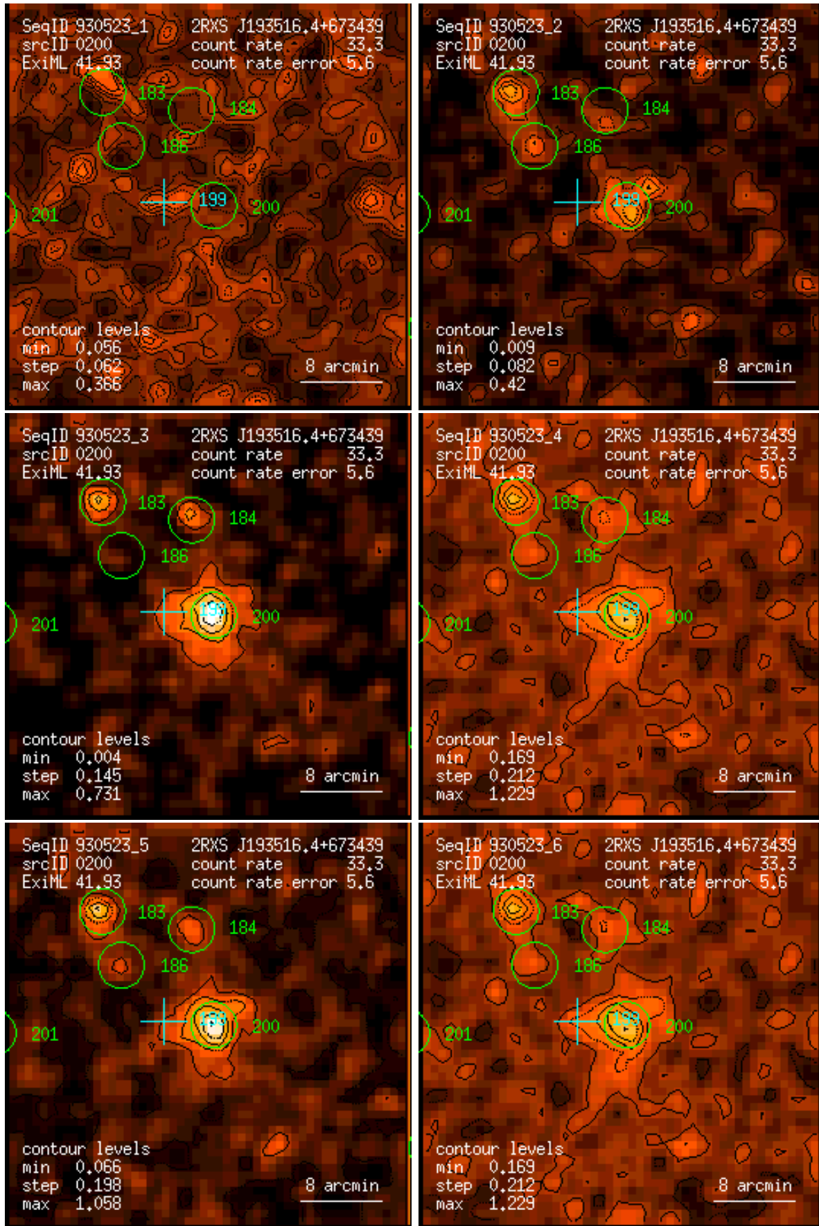
Figure 200: RASS 930523: detection 0200: band rate images, Gaussian filter: (1) PSPC channels 11 – 41, (2) 52 – 90, (3) 91 – 201, (4) 11 – 235, (5) 52 – 201, (6) 11 – 201. Broad band rates in counts/ks. Band rate contour levels in counts/ks/arcmin 2 .
