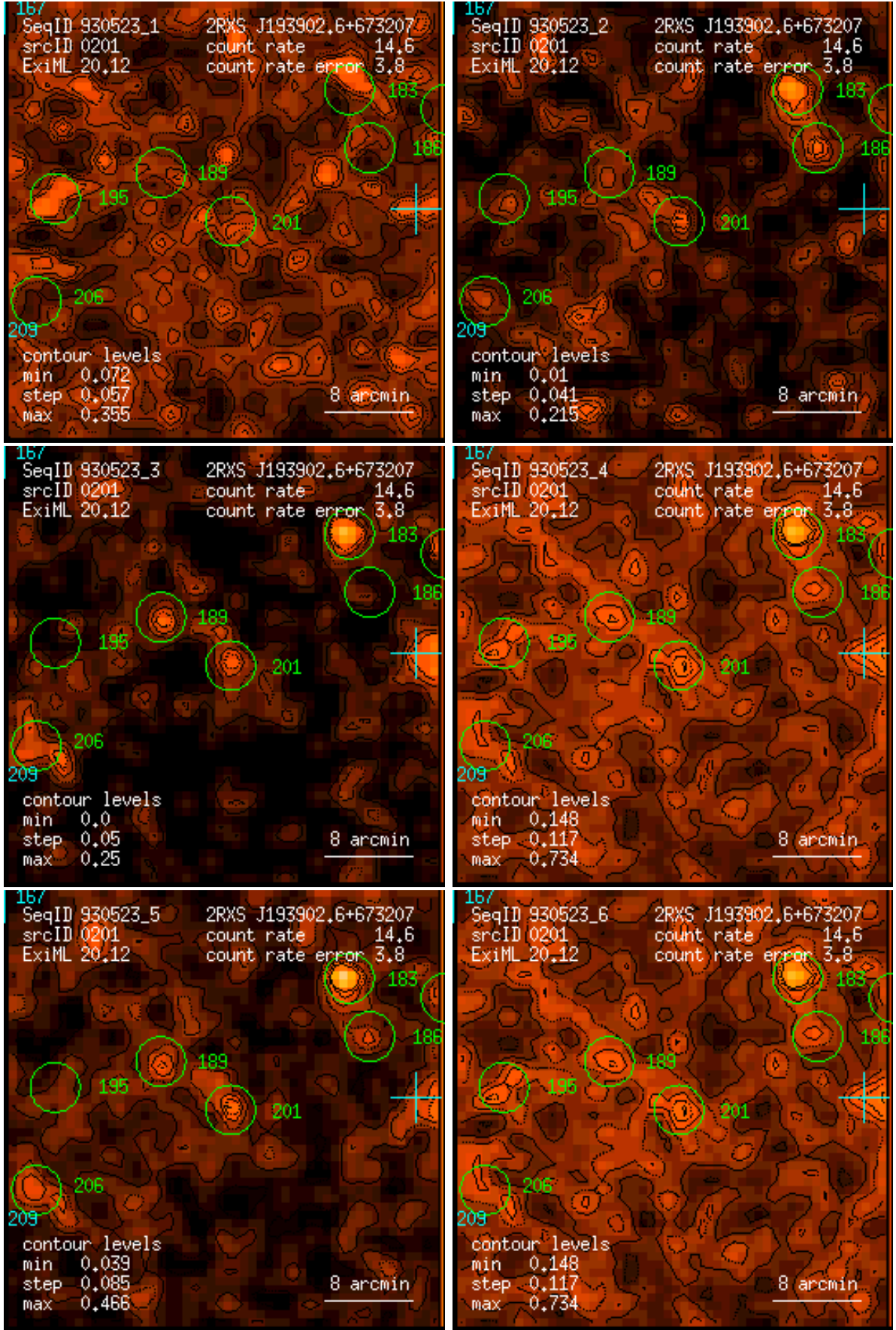
Figure 201: RASS 930523: detection 0201: band rate images, Gaussian filter: (1) PSPC channels 11 – 41, (2) 52 – 90, (3) 91 – 201, (4) 11 – 235, (5) 52 – 201, (6) 11 – 201. Broad band rates in counts/ks. Band rate contour levels in counts/ks/arcmin 2 .
