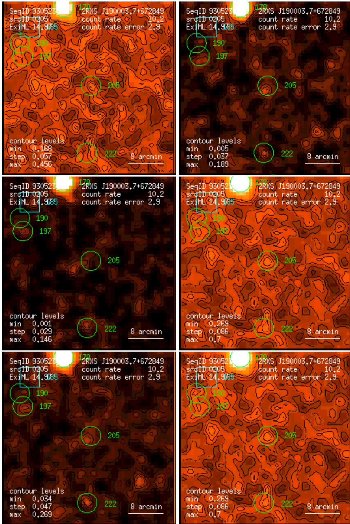
Figure 205: RASS 930523: detection 0205: band rate images, Gaussian filter: (1) PSPC channels 11 – 41, (2) 52 – 90, (3) 91 – 201, (4) 11 – 235, (5) 52 – 201, (6) 11 – 201. Broad band rates in counts/ks. Band rate contour levels in counts/ks/arcmin 2 .
