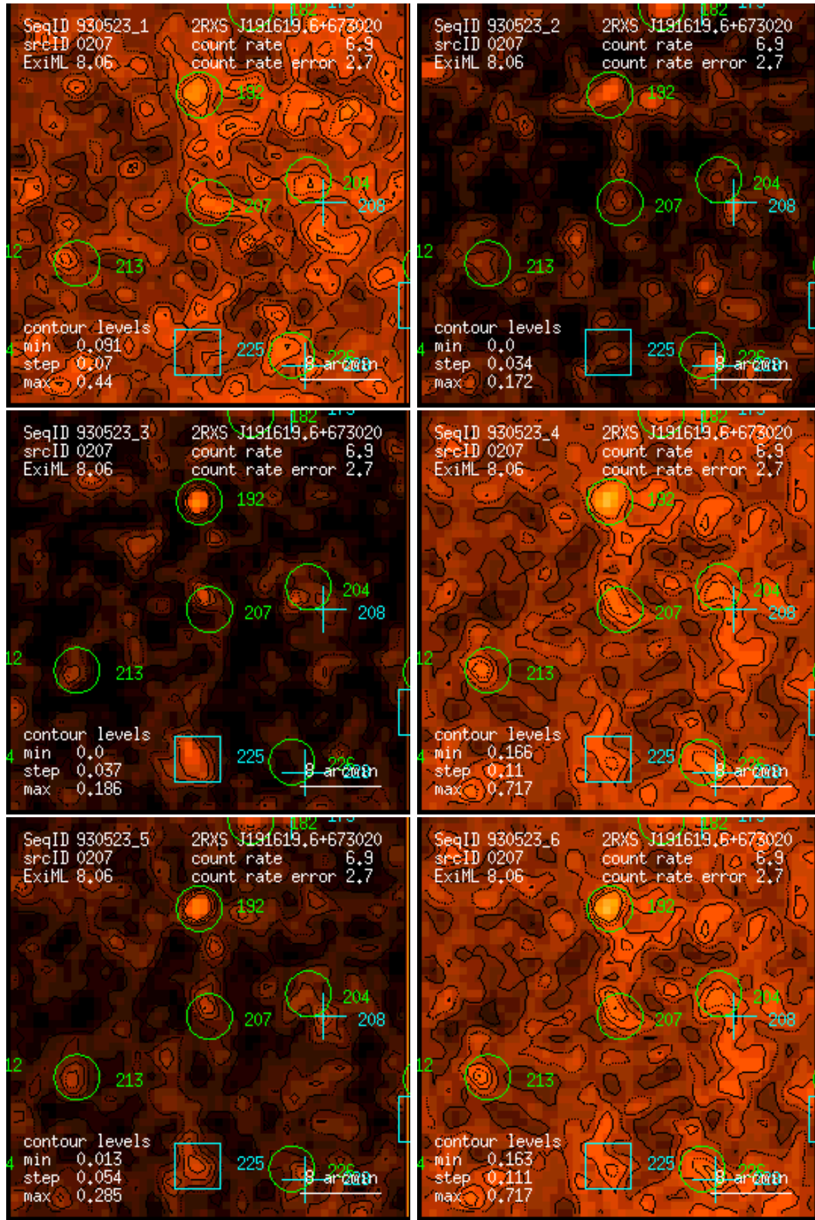
Figure 207: RASS 930523: detection 0207: band rate images, Gaussian filter: (1) PSPC channels 11 – 41, (2) 52 – 90, (3) 91 – 201, (4) 11 – 235, (5) 52 – 201, (6) 11 – 201. Broad band rates in counts/ks. Band rate contour levels in counts/ks/arcmin 2 .
