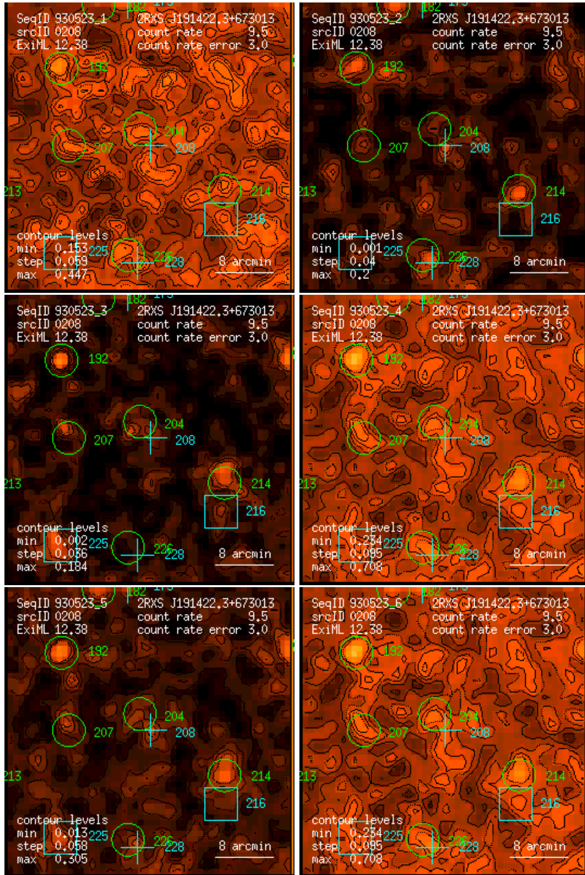
Figure 208: RASS 930523: detection 0208: band rate images, Gaussian filter: (1) PSPC channels 11 – 41, (2) 52 – 90, (3) 91 – 201, (4) 11 – 235, (5) 52 – 201, (6) 11 – 201. Broad band rates in counts/ks. Band rate contour levels in counts/ks/arcmin 2 .
