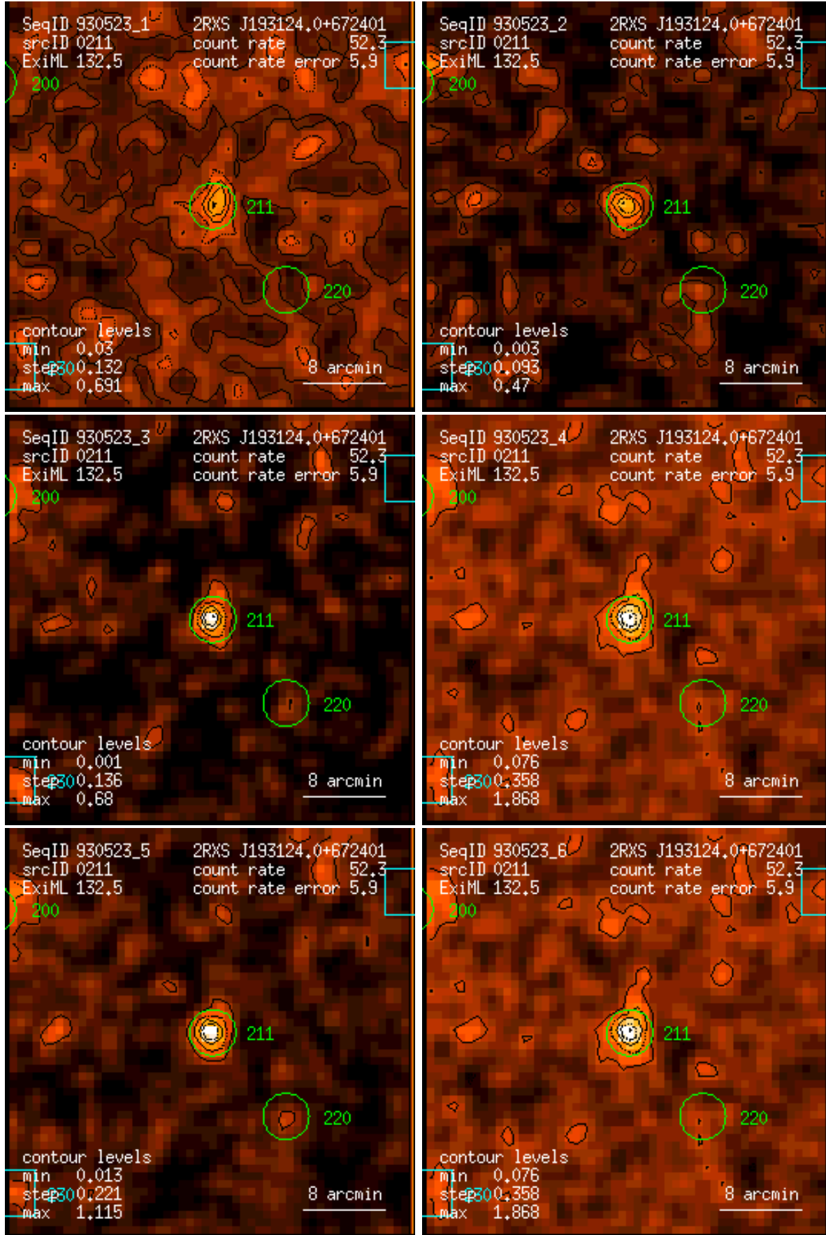
Figure 211: RASS 930523: detection 0211: band rate images, Gaussian filter: (1) PSPC channels 11 – 41, (2) 52 – 90, (3) 91 – 201, (4) 11 – 235, (5) 52 – 201, (6) 11 – 201. Broad band rates in counts/ks. Band rate contour levels in counts/ks/arcmin 2 .
