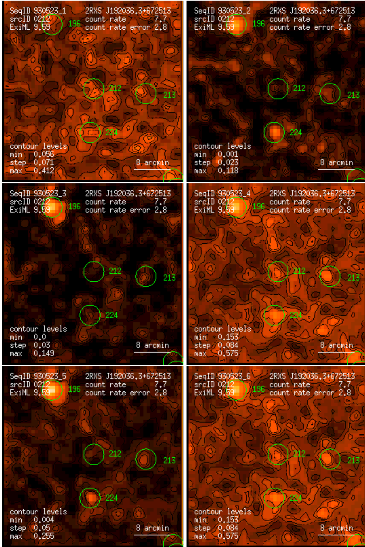
Figure 212: RASS 930523: detection 0212: band rate images, Gaussian filter: (1) PSPC channels 11 – 41, (2) 52 – 90, (3) 91 – 201, (4) 11 – 235, (5) 52 – 201, (6) 11 – 201. Broad band rates in counts/ks. Band rate contour levels in counts/ks/arcmin 2 .
