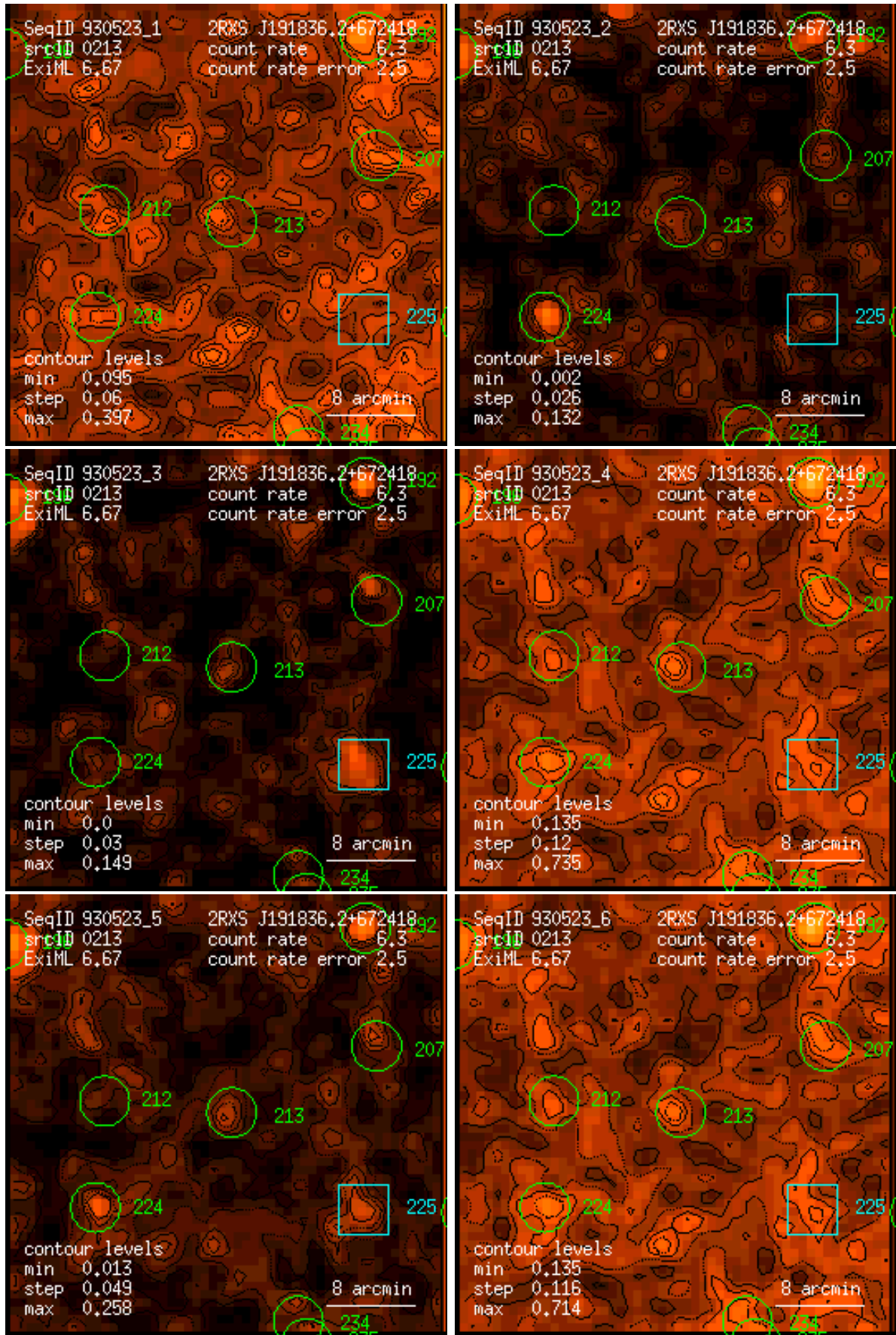
Figure 213: RASS 930523: detection 0213: band rate images, Gaussian filter: (1) PSPC channels 11 – 41, (2) 52 – 90, (3) 91 – 201, (4) 11 – 235, (5) 52 – 201, (6) 11 – 201. Broad band rates in counts/ks. Band rate contour levels in counts/ks/arcmin 2 .
