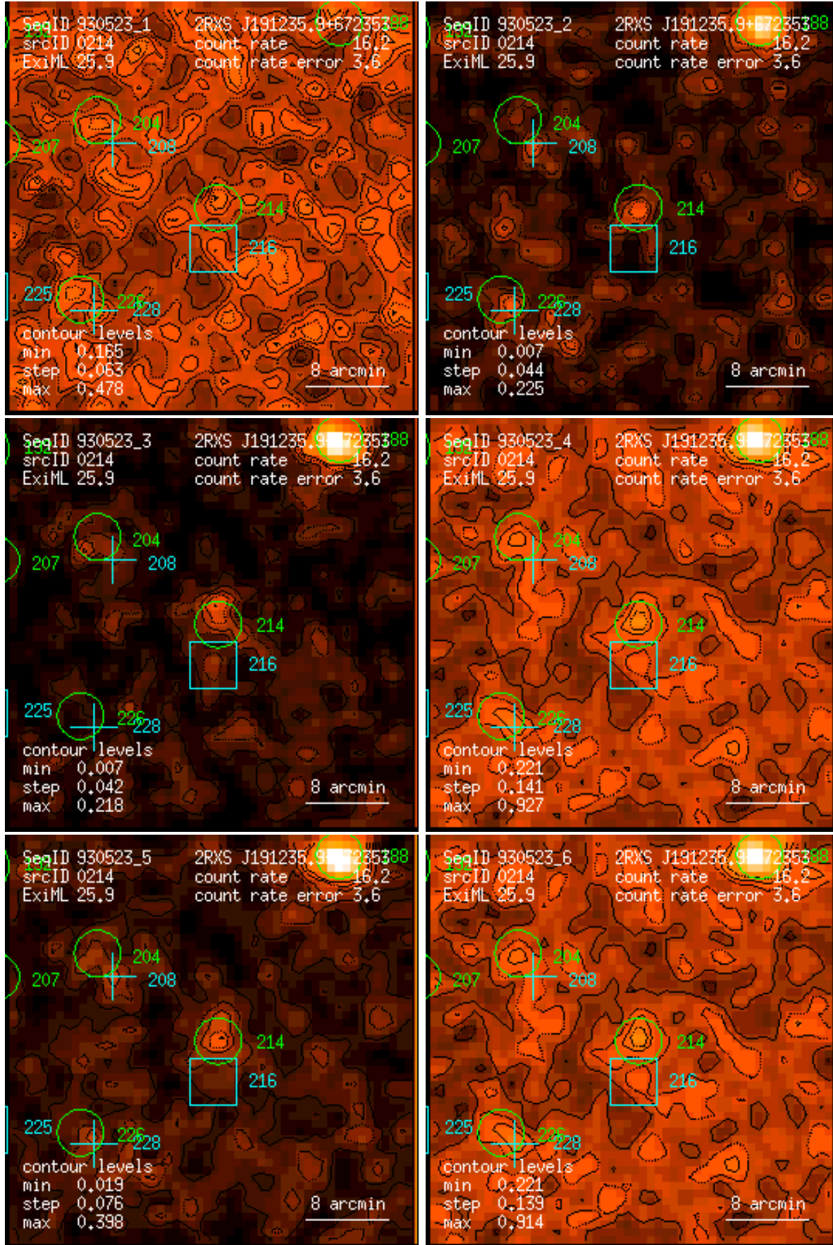
Figure 214: RASS 930523: detection 0214: band rate images, Gaussian filter: (1) PSPC channels 11 – 41, (2) 52 – 90, (3) 91 – 201, (4) 11 – 235, (5) 52 – 201, (6) 11 – 201. Broad band rates in counts/ks. Band rate contour levels in counts/ks/arcmin 2 .
