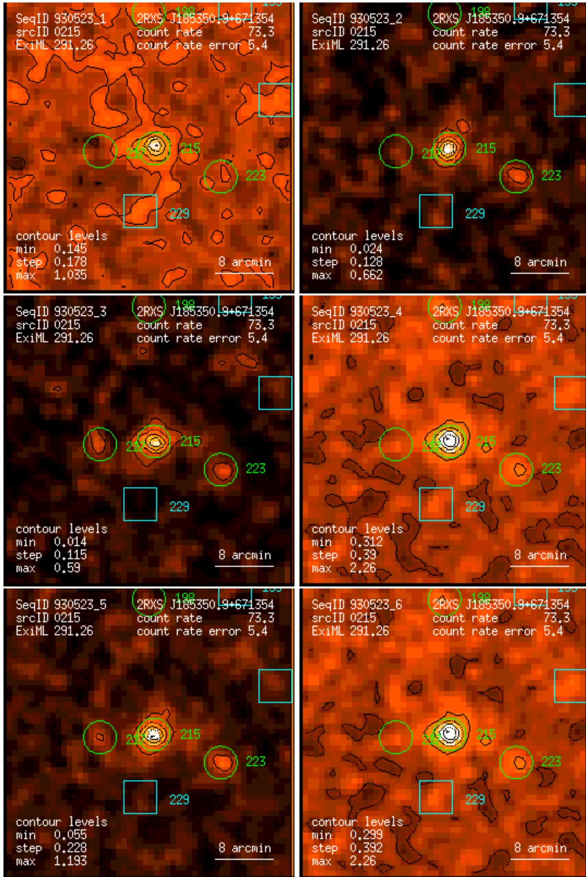
Figure 215: RASS 930523: detection 0215: band rate images, Gaussian filter: (1) PSPC channels 11 – 41, (2) 52 – 90, (3) 91 – 201, (4) 11 – 235, (5) 52 – 201, (6) 11 – 201. Broad band rates in counts/ks. Band rate contour levels in counts/ks/arcmin 2 .
