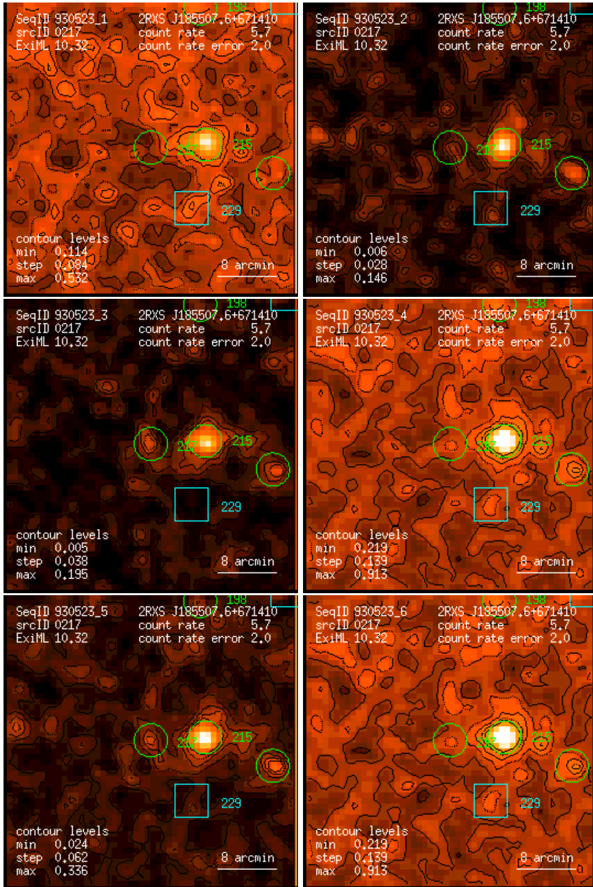
Figure 217: RASS 930523: detection 0217: band rate images, Gaussian filter: (1) PSPC channels 11 – 41, (2) 52 – 90, (3) 91 – 201, (4) 11 – 235, (5) 52 – 201, (6) 11 – 201. Broad band rates in counts/ks. Band rate contour levels in counts/ks/arcmin 2 .
