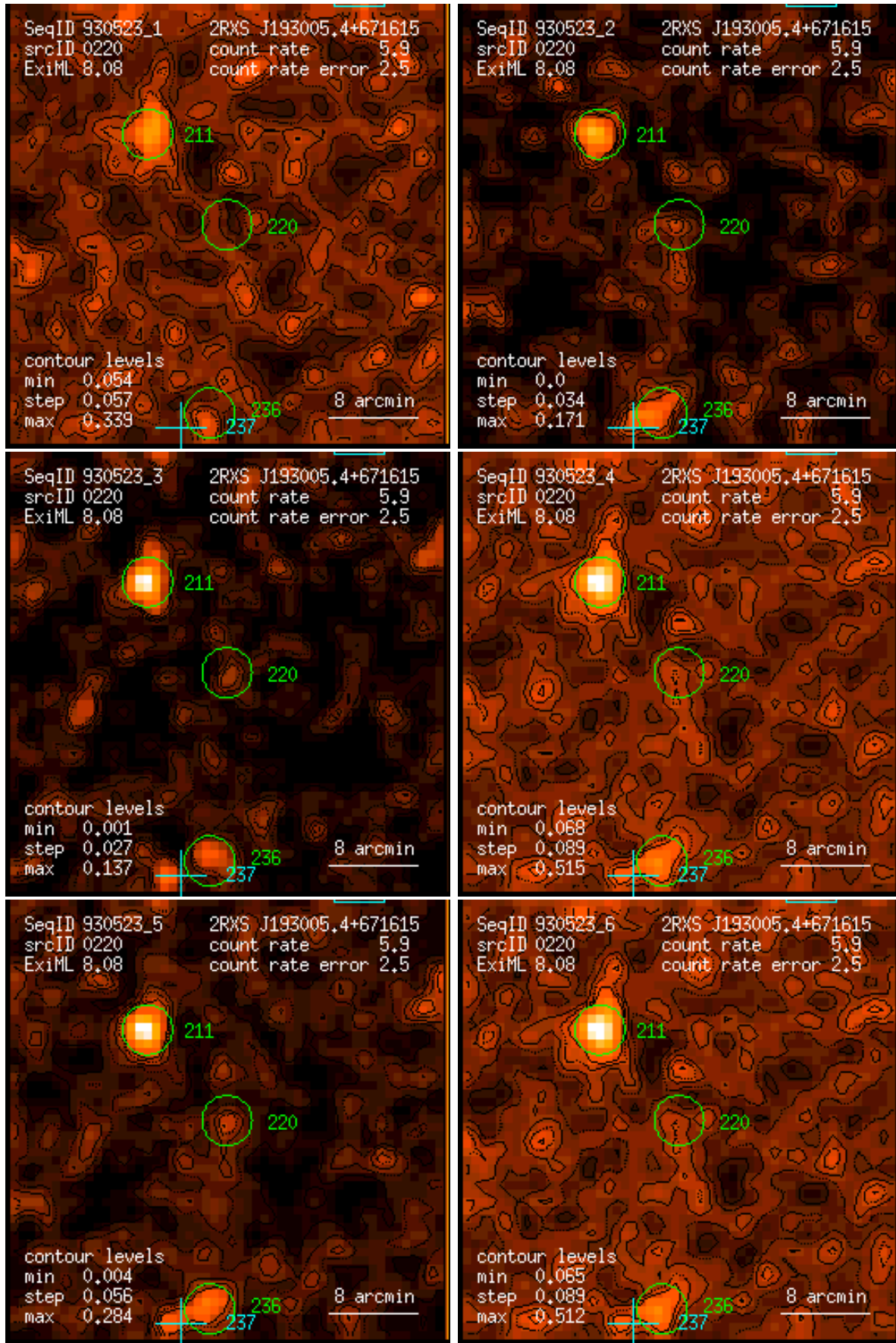
Figure 220: RASS 930523: detection 0220: band rate images, Gaussian filter: (1) PSPC channels 11 – 41, (2) 52 – 90, (3) 91 – 201, (4) 11 – 235, (5) 52 – 201, (6) 11 – 201. Broad band rates in counts/ks. Band rate contour levels in counts/ks/arcmin 2 .
