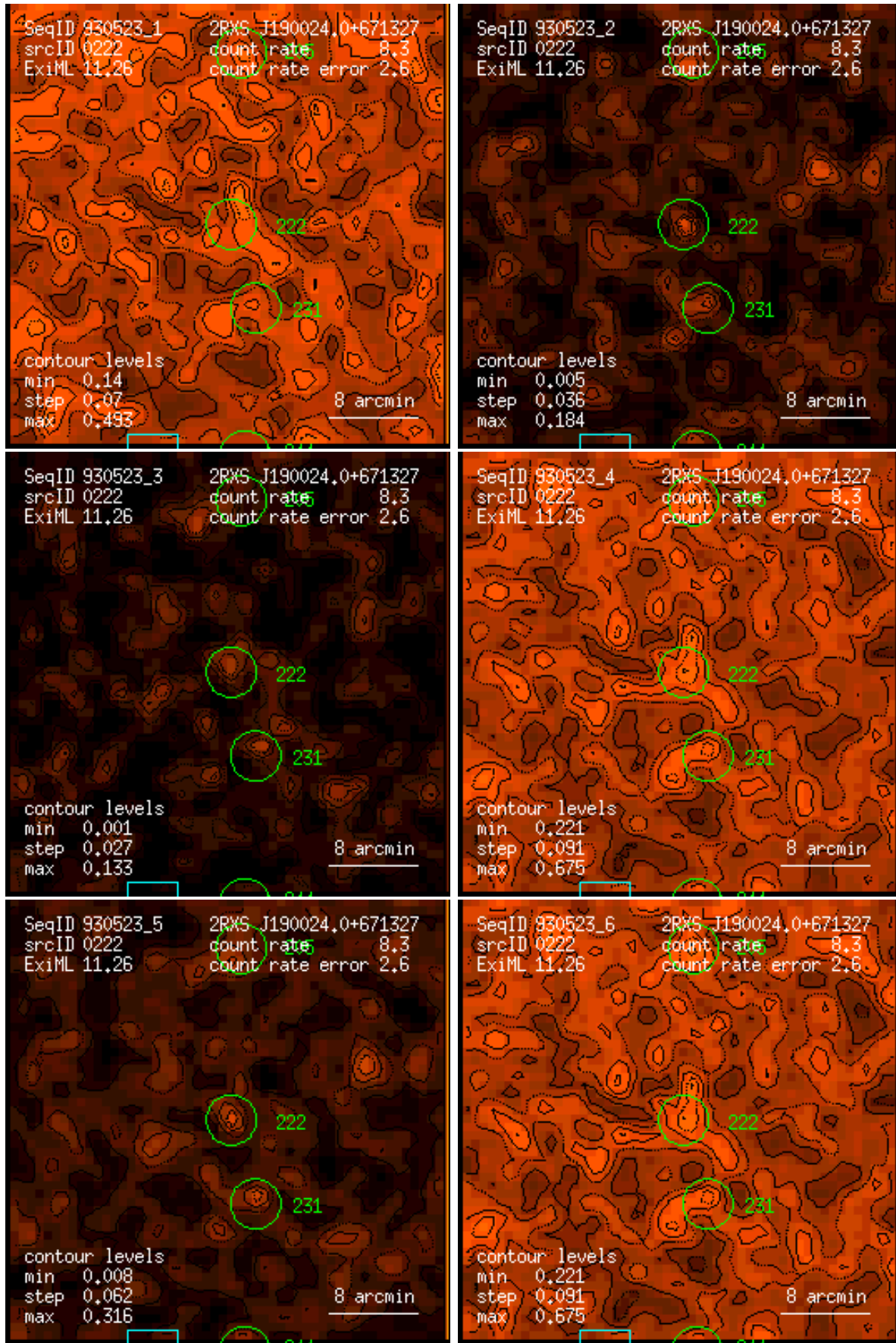
Figure 222: RASS 930523: detection 0222: band rate images, Gaussian filter: (1) PSPC channels 11 – 41, (2) 52 – 90, (3) 91 – 201, (4) 11 – 235, (5) 52 – 201, (6) 11 – 201. Broad band rates in counts/ks. Band rate contour levels in counts/ks/arcmin 2 .
