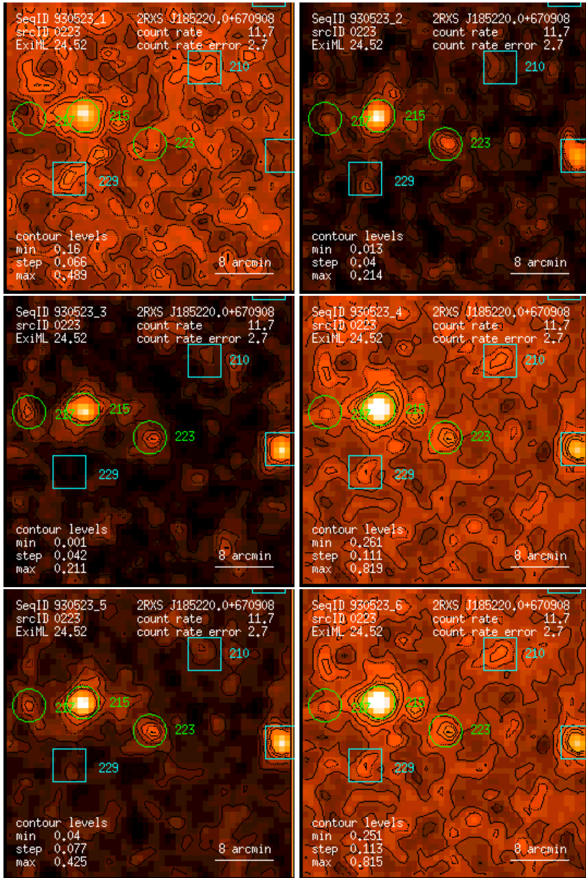
Figure 223: RASS 930523: detection 0223: band rate images, Gaussian filter: (1) PSPC channels 11 – 41, (2) 52 – 90, (3) 91 – 201, (4) 11 – 235, (5) 52 – 201, (6) 11 – 201. Broad band rates in counts/ks. Band rate contour levels in counts/ks/arcmin 2 .
