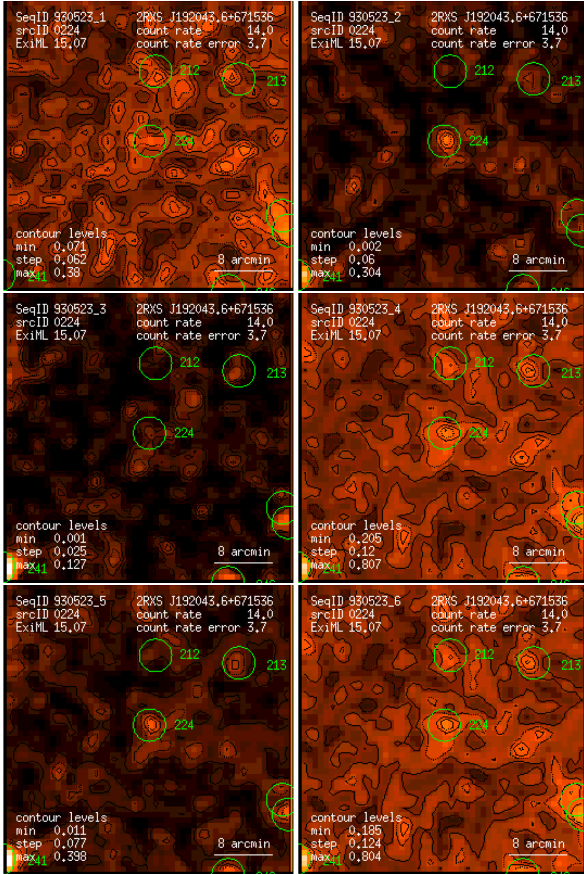
Figure 224: RASS 930523: detection 0224: band rate images, Gaussian filter: (1) PSPC channels 11 – 41, (2) 52 – 90, (3) 91 – 201, (4) 11 – 235, (5) 52 – 201, (6) 11 – 201. Broad band rates in counts/ks. Band rate contour levels in counts/ks/arcmin 2 .
