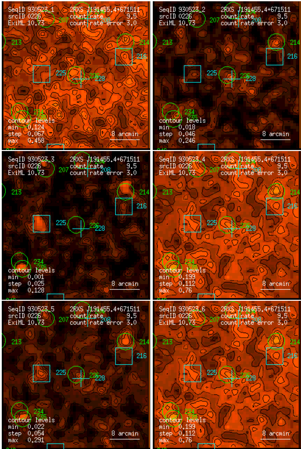
Figure 226: RASS 930523: detection 0226: band rate images, Gaussian filter: (1) PSPC channels 11 – 41, (2) 52 – 90, (3) 91 – 201, (4) 11 – 235, (5) 52 – 201, (6) 11 – 201. Broad band rates in counts/ks. Band rate contour levels in counts/ks/arcmin 2 .
