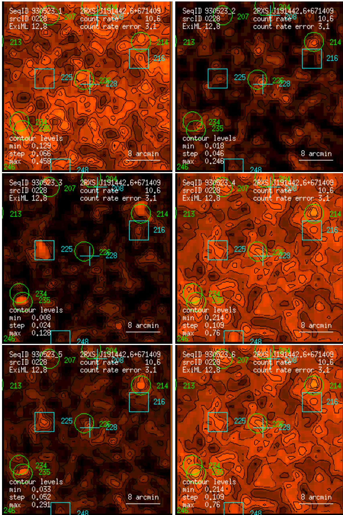
Figure 228: RASS 930523: detection 0228: band rate images, Gaussian filter: (1) PSPC channels 11 – 41, (2) 52 – 90, (3) 91 – 201, (4) 11 – 235, (5) 52 – 201, (6) 11 – 201. Broad band rates in counts/ks. Band rate contour levels in counts/ks/arcmin 2 .
