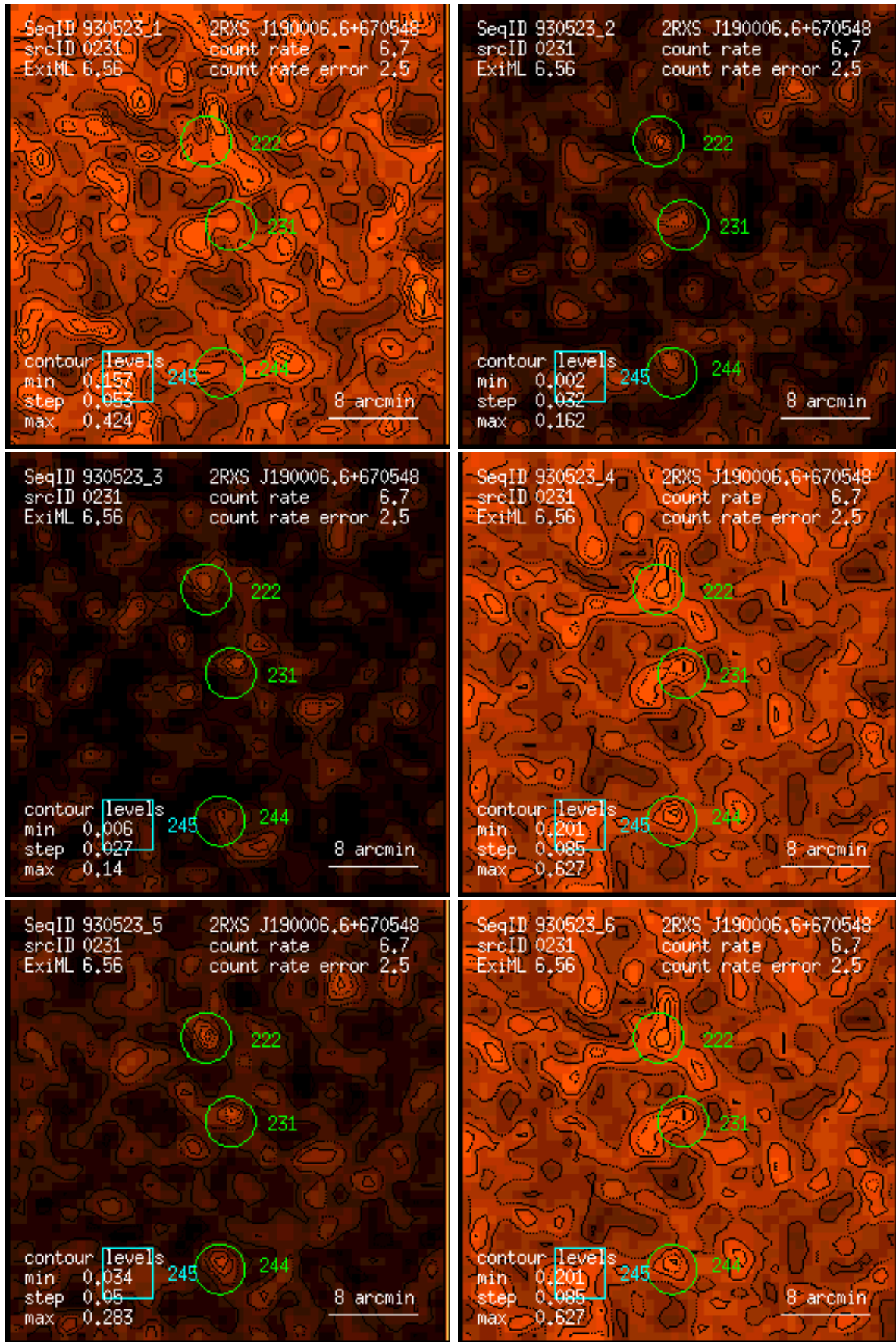
Figure 231: RASS 930523: detection 0231: band rate images, Gaussian filter: (1) PSPC channels 11 – 41, (2) 52 – 90, (3) 91 – 201, (4) 11 – 235, (5) 52 – 201, (6) 11 – 201. Broad band rates in counts/ks. Band rate contour levels in counts/ks/arcmin 2 .
