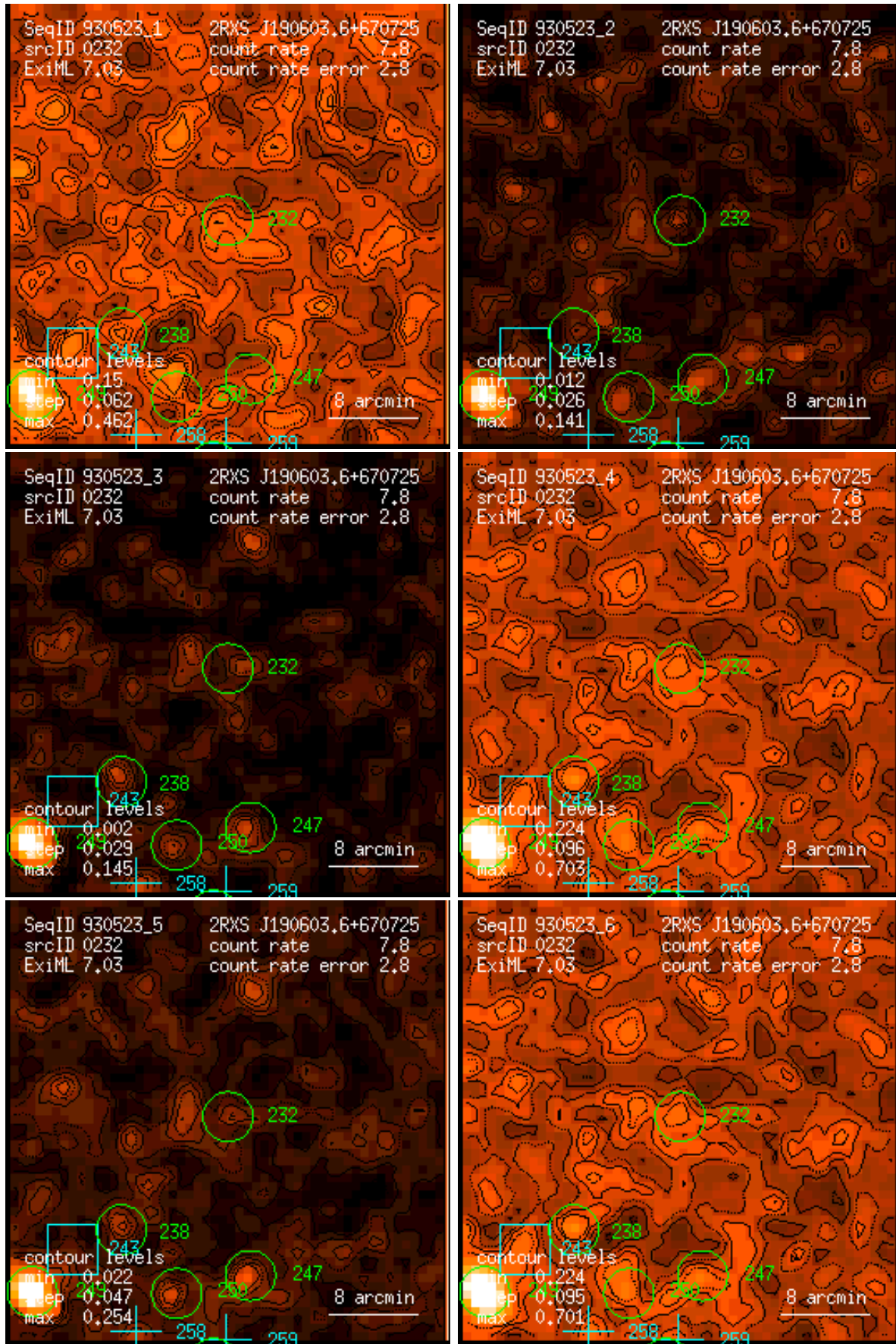
Figure 232: RASS 930523: detection 0232: band rate images, Gaussian filter: (1) PSPC channels 11 – 41, (2) 52 – 90, (3) 91 – 201, (4) 11 – 235, (5) 52 – 201, (6) 11 – 201. Broad band rates in counts/ks. Band rate contour levels in counts/ks/arcmin 2 .
