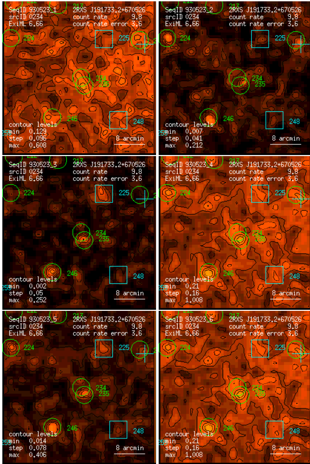
Figure 234: RASS 930523: detection 0234: band rate images, Gaussian filter: (1) PSPC channels 11 – 41, (2) 52 – 90, (3) 91 – 201, (4) 11 – 235, (5) 52 – 201, (6) 11 – 201. Broad band rates in counts/ks. Band rate contour levels in counts/ks/arcmin 2 .
