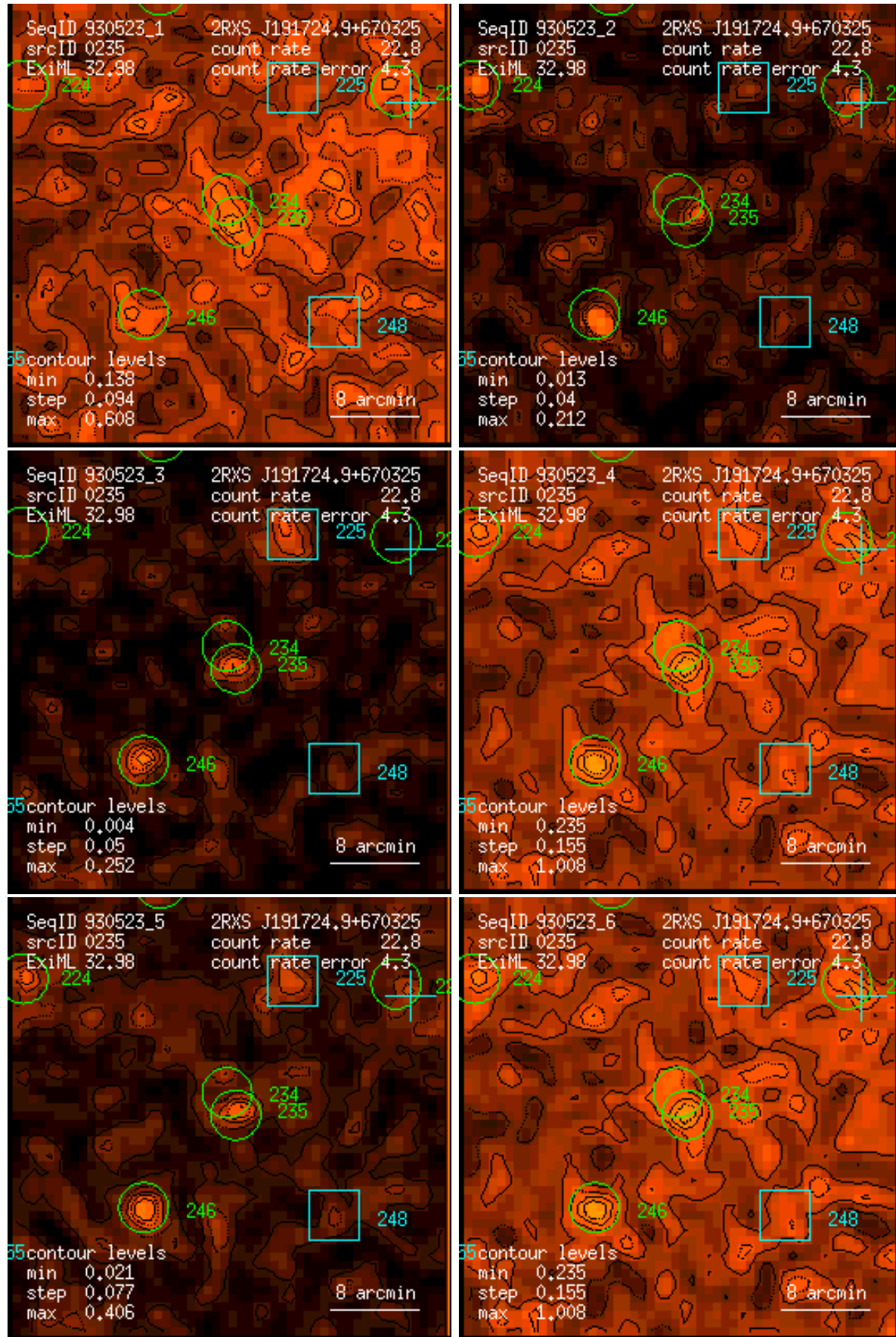
Figure 235: RASS 930523: detection 0235: band rate images, Gaussian filter: (1) PSPC channels 11 – 41, (2) 52 – 90, (3) 91 – 201, (4) 11 – 235, (5) 52 – 201, (6) 11 – 201. Broad band rates in counts/ks. Band rate contour levels in counts/ks/arcmin 2 .
