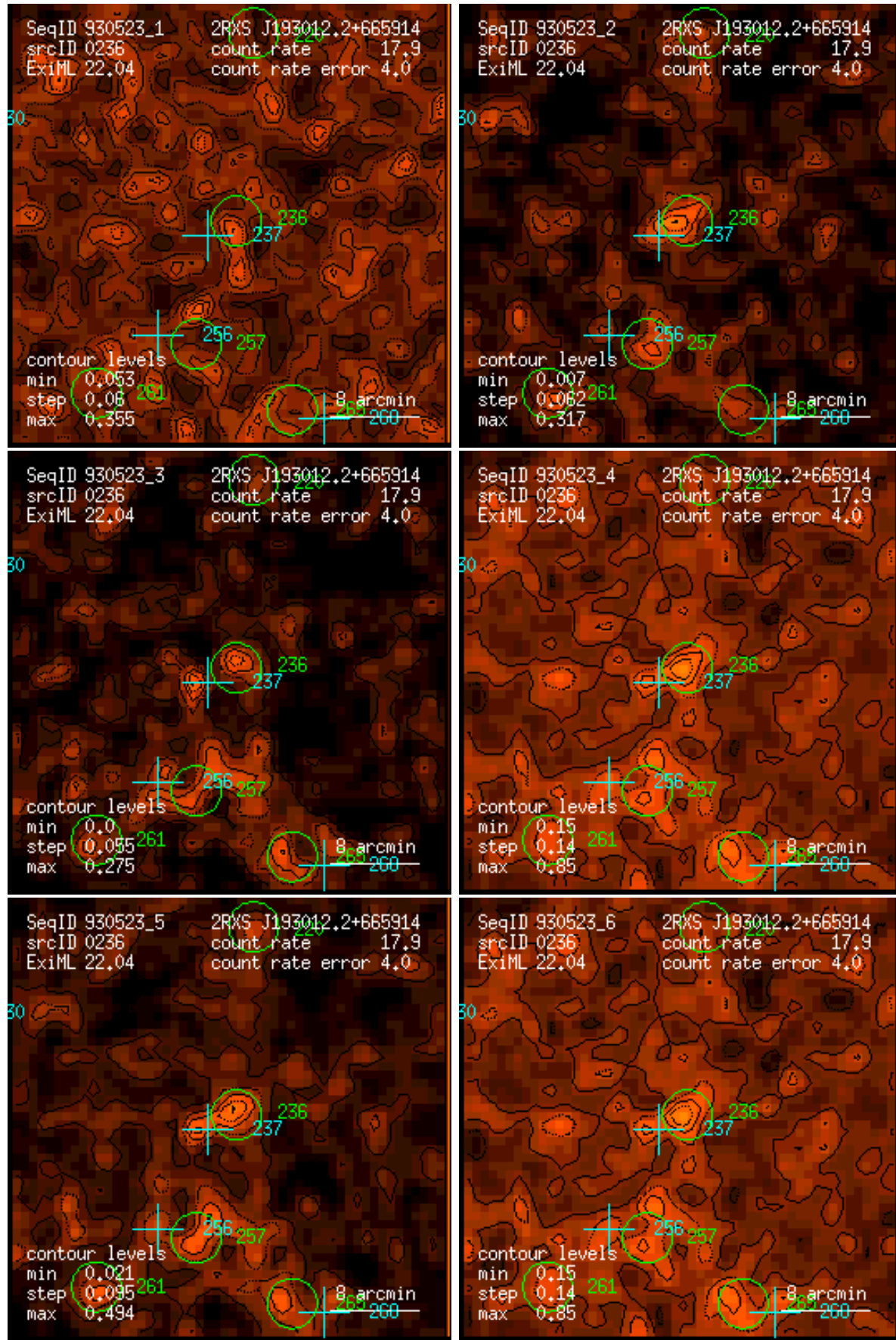
Figure 236: RASS 930523: detection 0236: band rate images, Gaussian filter: (1) PSPC channels 11 – 41, (2) 52 – 90, (3) 91 – 201, (4) 11 – 235, (5) 52 – 201, (6) 11 – 201. Broad band rates in counts/ks. Band rate contour levels in counts/ks/arcmin 2 .
