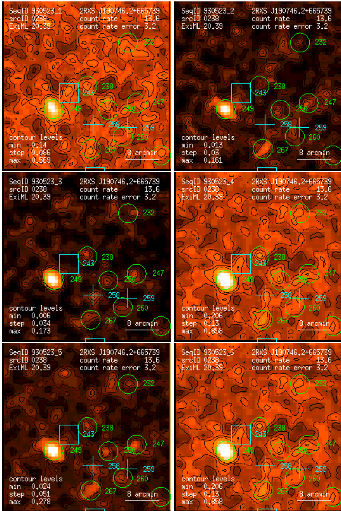
Figure 238: RASS 930523: detection 0238: band rate images, Gaussian filter: (1) PSPC channels 11 – 41, (2) 52 – 90, (3) 91 – 201, (4) 11 – 235, (5) 52 – 201, (6) 11 – 201. Broad band rates in counts/ks. Band rate contour levels in counts/ks/arcmin 2 .
