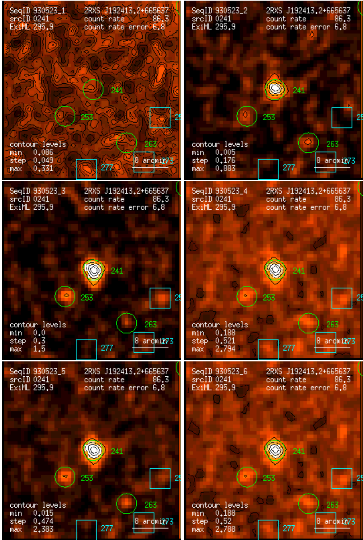
Figure 241: RASS 930523: detection 0241: band rate images, Gaussian filter: (1) PSPC channels 11 – 41, (2) 52 – 90, (3) 91 – 201, (4) 11 – 235, (5) 52 – 201, (6) 11 – 201. Broad band rates in counts/ks. Band rate contour levels in counts/ks/arcmin 2 .
