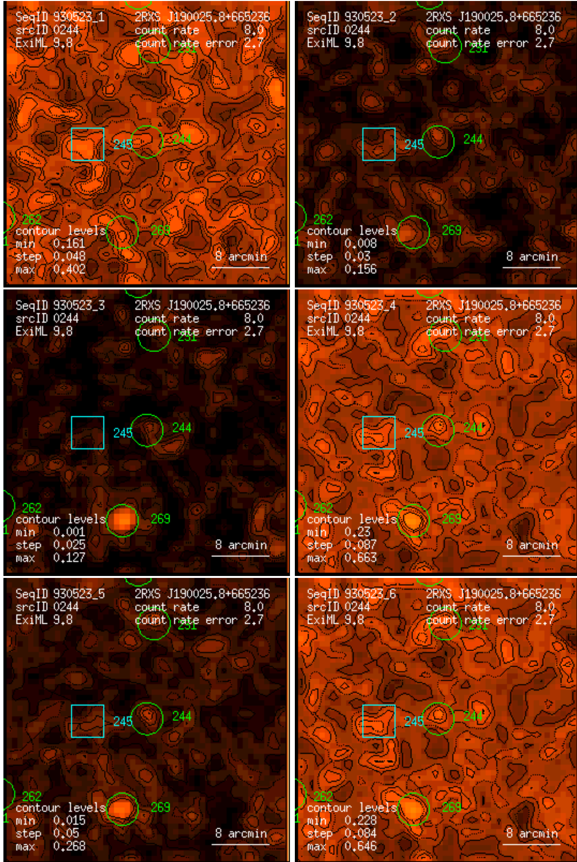
Figure 244: RASS 930523: detection 0244: band rate images, Gaussian filter: (1) PSPC channels 11 – 41, (2) 52 – 90, (3) 91 – 201, (4) 11 – 235, (5) 52 – 201, (6) 11 – 201. Broad band rates in counts/ks. Band rate contour levels in counts/ks/arcmin 2 .
