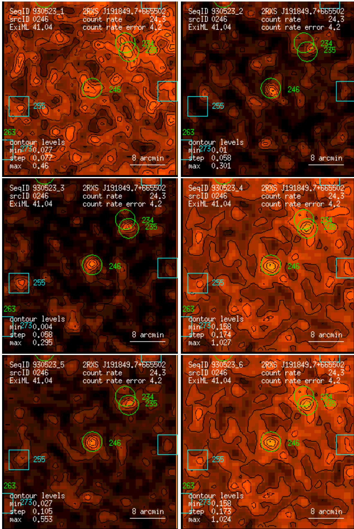
Figure 246: RASS 930523: detection 0246: band rate images, Gaussian filter: (1) PSPC channels 11 – 41, (2) 52 – 90, (3) 91 – 201, (4) 11 – 235, (5) 52 – 201, (6) 11 – 201. Broad band rates in counts/ks. Band rate contour levels in counts/ks/arcmin 2 .
