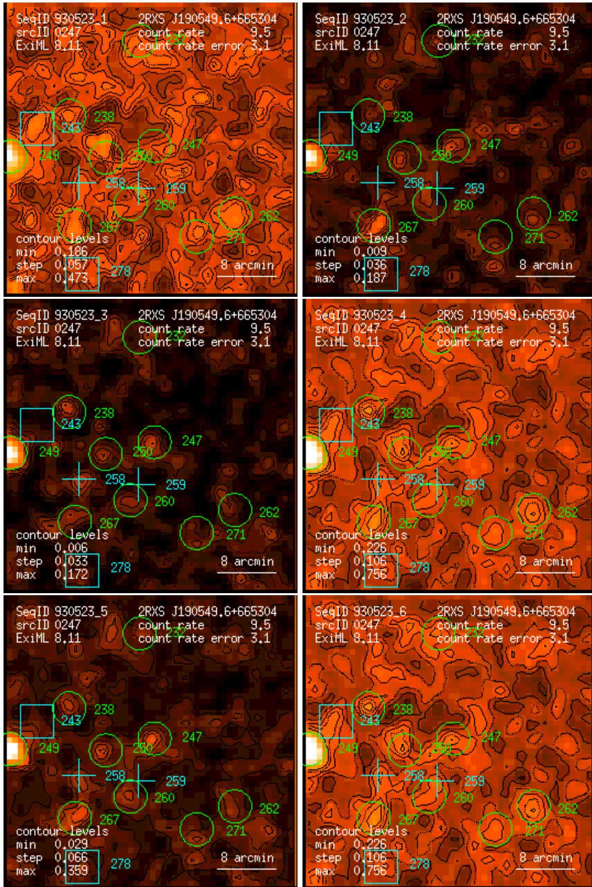
Figure 247: RASS 930523: detection 0247: band rate images, Gaussian filter: (1) PSPC channels 11 – 41, (2) 52 – 90, (3) 91 – 201, (4) 11 – 235, (5) 52 – 201, (6) 11 – 201. Broad band rates in counts/ks. Band rate contour levels in counts/ks/arcmin 2 .
