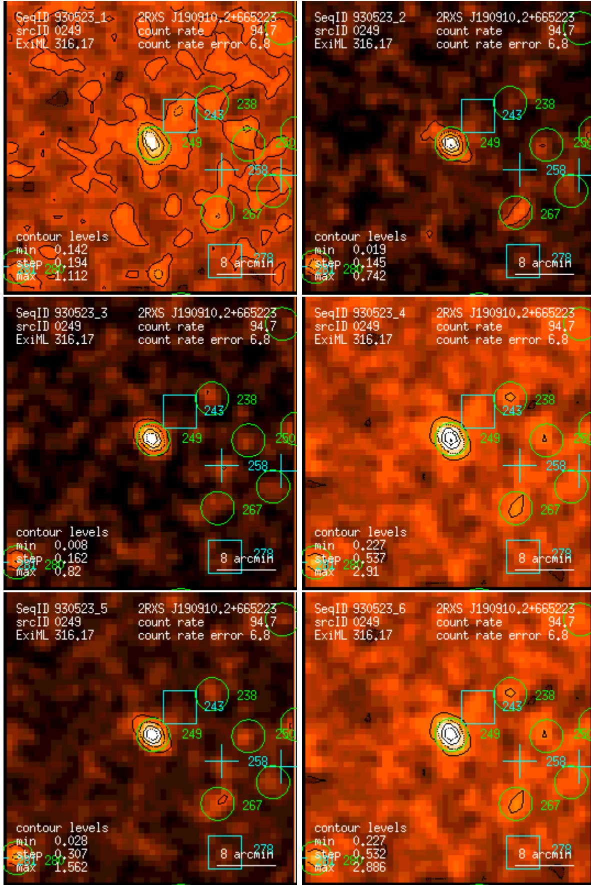
Figure 249: RASS 930523: detection 0249: band rate images, Gaussian filter: (1) PSPC channels 11 – 41, (2) 52 – 90, (3) 91 – 201, (4) 11 – 235, (5) 52 – 201, (6) 11 – 201. Broad band rates in counts/ks. Band rate contour levels in counts/ks/arcmin 2 .
