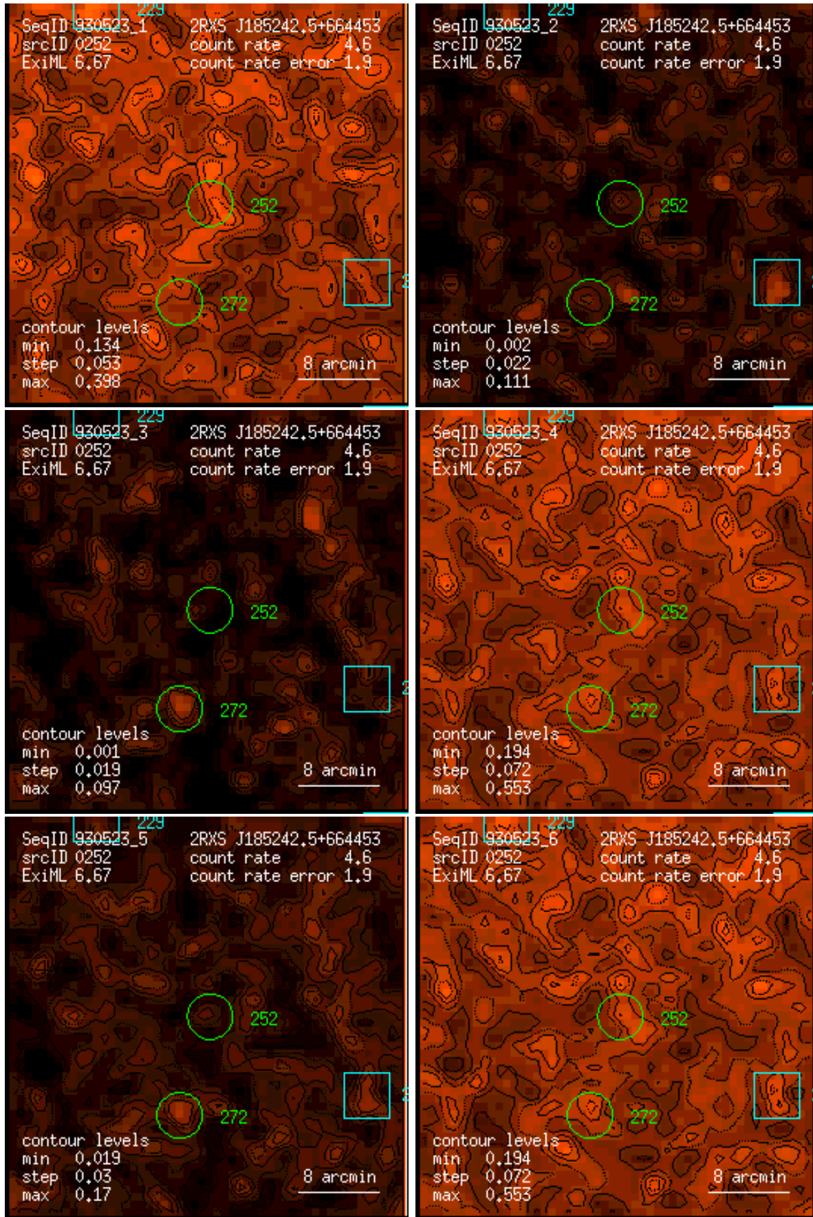
Figure 252: RASS 930523: detection 0252: band rate images, Gaussian filter: (1) PSPC channels 11 – 41, (2) 52 – 90, (3) 91 – 201, (4) 11 – 235, (5) 52 – 201, (6) 11 – 201. Broad band rates in counts/ks. Band rate contour levels in counts/ks/arcmin 2 .
