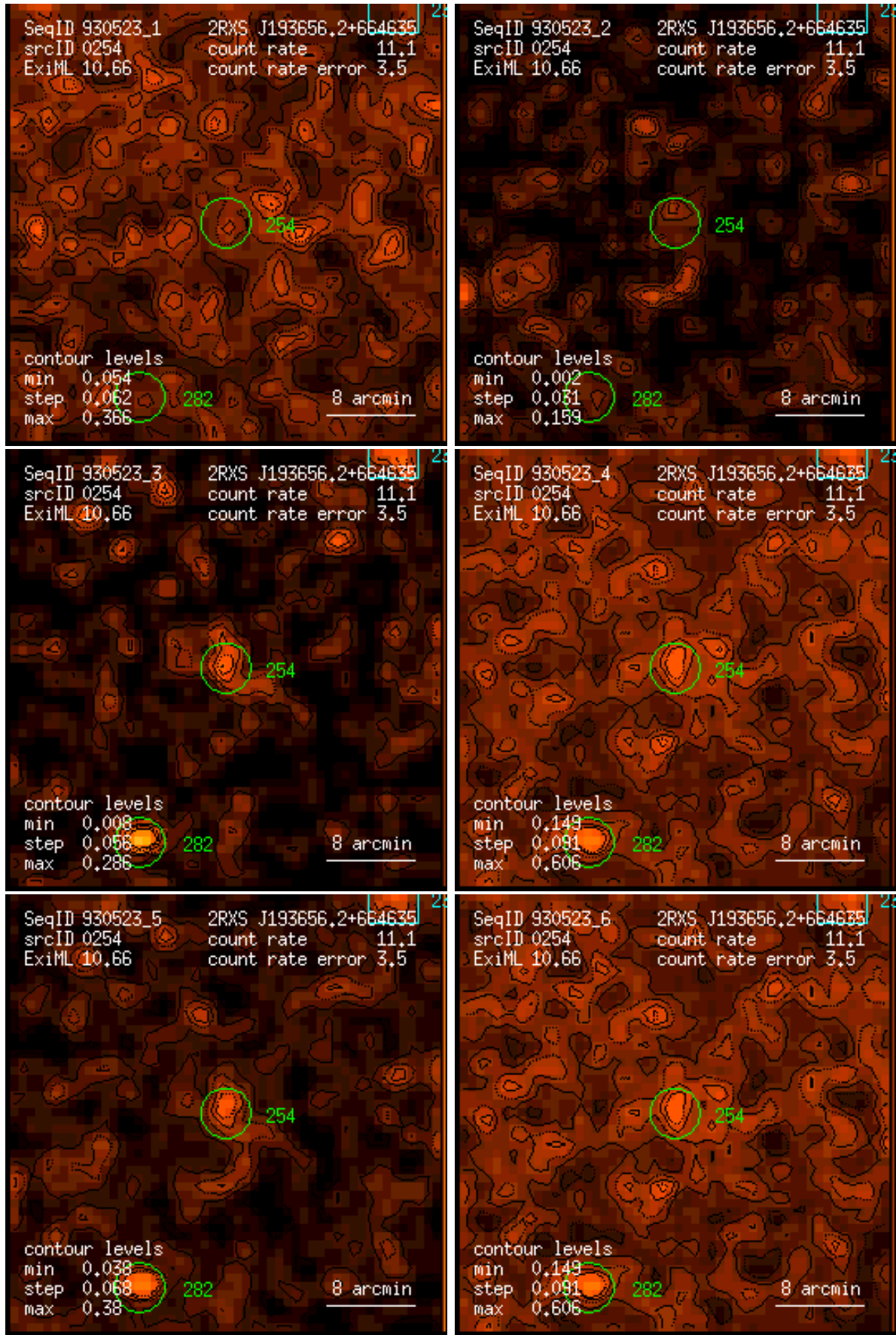
Figure 254: RASS 930523: detection 0254: band rate images, Gaussian filter: (1) PSPC channels 11 – 41, (2) 52 – 90, (3) 91 – 201, (4) 11 – 235, (5) 52 – 201, (6) 11 – 201. Broad band rates in counts/ks. Band rate contour levels in counts/ks/arcmin 2 .
