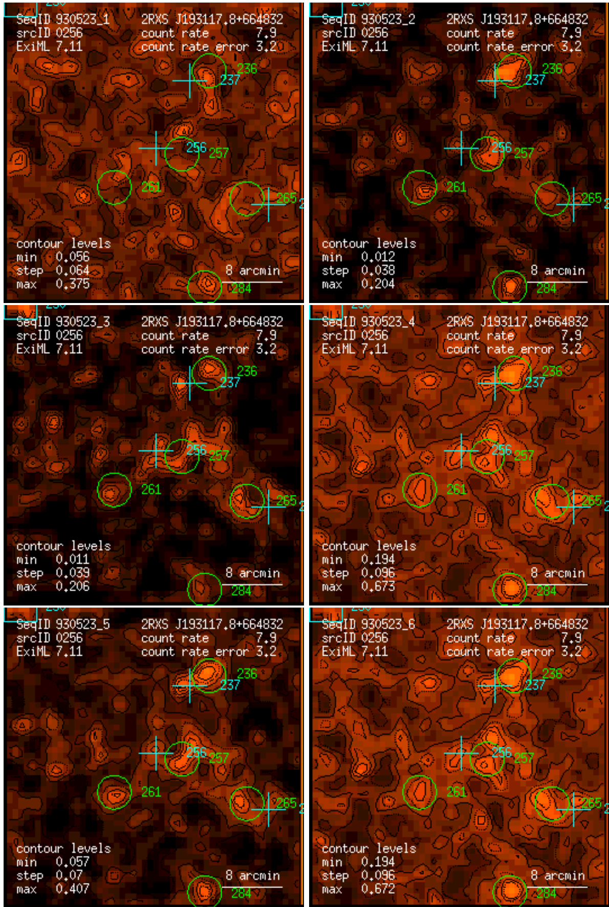
Figure 256: RASS 930523: detection 0256: band rate images, Gaussian filter: (1) PSPC channels 11 – 41, (2) 52 – 90, (3) 91 – 201, (4) 11 – 235, (5) 52 – 201, (6) 11 – 201. Broad band rates in counts/ks. Band rate contour levels in counts/ks/arcmin 2 .
