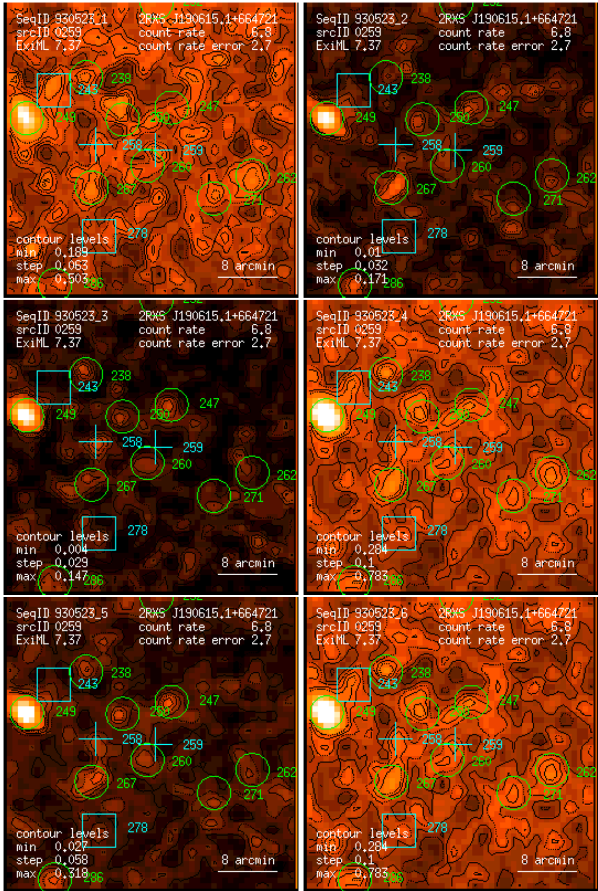
Figure 259: RASS 930523: detection 0259: band rate images, Gaussian filter: (1) PSPC channels 11 – 41, (2) 52 – 90, (3) 91 – 201, (4) 11 – 235, (5) 52 – 201, (6) 11 – 201. Broad band rates in counts/ks. Band rate contour levels in counts/ks/arcmin 2 .
